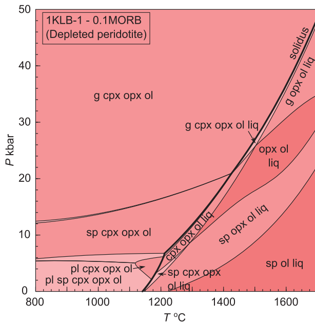
Fig. 5. P - T pseudosection for the depleted peridotite bulk composition X = -0.1 (KLB-1 - 0.1N-MORB), in the NCFMASOC system. Phase labels and legend as for Fig. 1.
