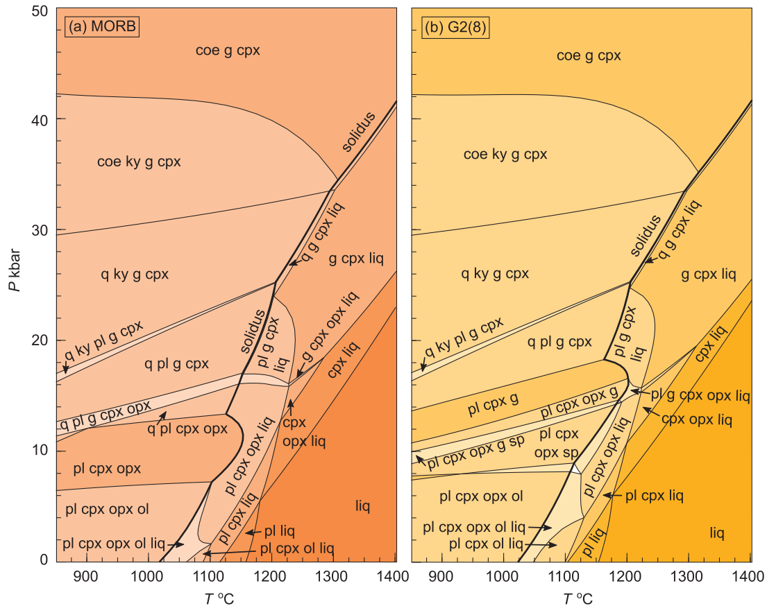
Fig. 3. P - T pseudosection calculated for (a) average MORB bulk composition of Gale et al. (2013) (N-MORB, Table 1 ) and (b) G2(8) eclogite bulk composition [ Table 1 ; after G2 composition of Pertermann & Hirschmann (2003a) ], both in the NCFMASOcr system with \text{Fe}^{3+}/\text{Fe}_T = 0.16 (after Cottrell & Kelley, 2011 ). Legend as for Fig. 1 ; additional phases: q, quartz; coe, coesite; ky, kyanite. Spinel is not present in (a).
