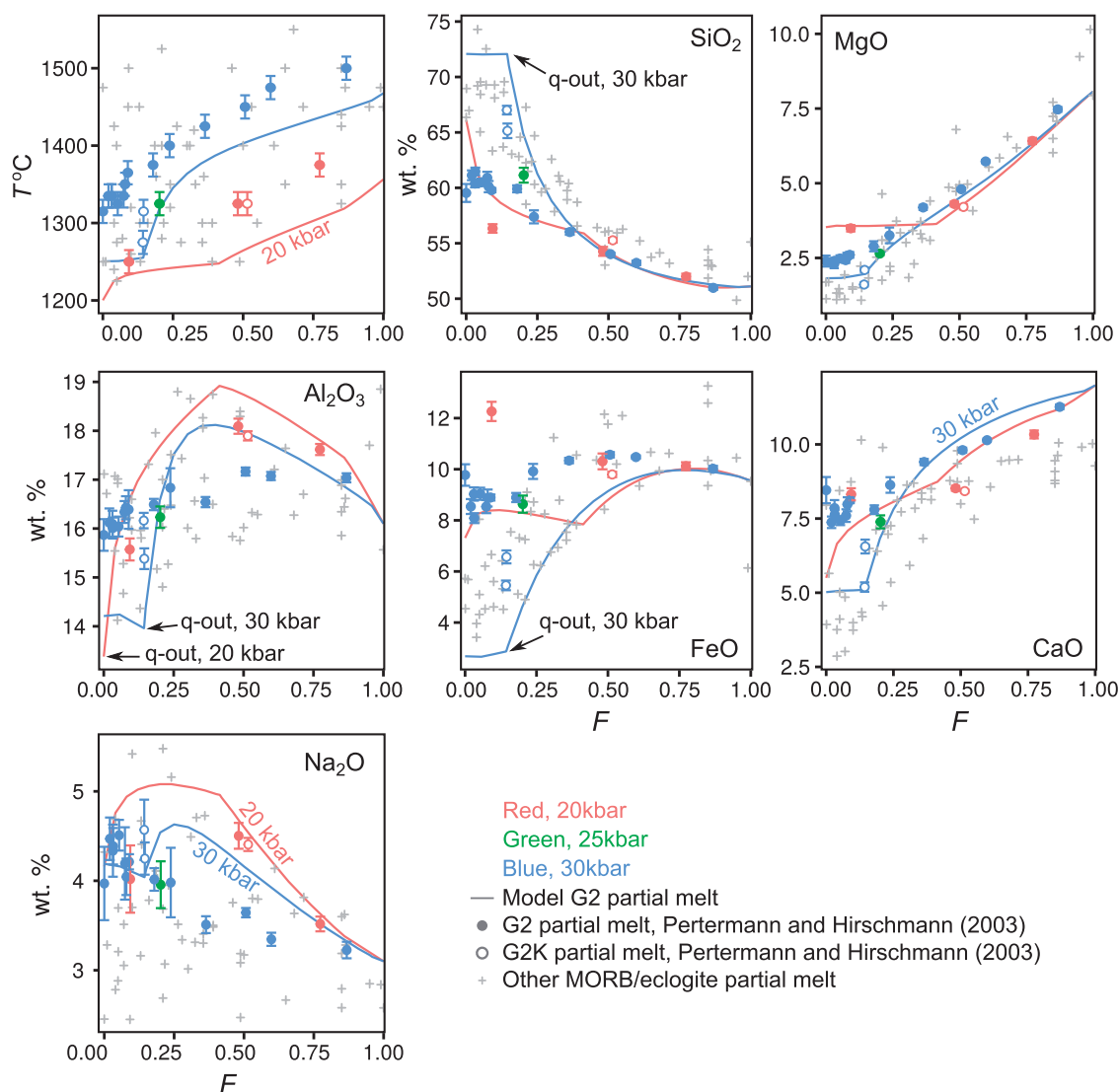
Fig. 4. Comparison of model melt compositions [lines, bulk composition G2(7)] with experiments of Pertermann & Hirschmann (2003a) for bulk composition G2 (experimental melts of G2K are also shown, which is a bulk composition somewhat higher in K_2O and SiO_2 than G2). Red, experiments and model at 20 kbar; green, 25 kbar; blue, 30 kbar. Experimental compositions and uncertainties are from Pertermann & Hirschmann (2003a) . The G2(7) bulk composition is ferric iron-free for comparability with experiments, which are buffered by graphite (see Table 1 ). q-out marks the exhaustion of quartz from the solid. Large differences in melt compositions at low F are explained by the presence or absence of quartz. Experimental melts from other studies using anhydrous eclogite compositions at a range of pressures are shown with grey crosses ( Takahashi et al. , 1998 ; Yaxley & Green, 1998 ; Takahashi & Nakajima, 2002 ; Yaxley & Sobolev, 2007 ; Spandler et al. , 2008 ; Rosenthal et al. , 2014 ).
