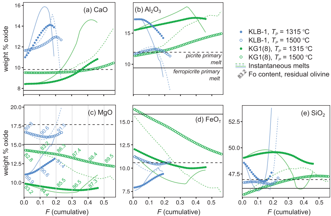
Fig. 12. Composition of accumulated fractional melts as a function of melt fraction F . (a) CaO, (b) \text{Al}_2\text{O}_3 , (c) MgO, (d) \text{FeO}_T and (e) \text{SiO}_2 , for polybaric fractional melting of peridotite KLB-1 (blue) and silica-deficient pyroxenite KG1(8) (green) and T_p = 1315 and 1500^\circ\text{C} . Each point represents an F = 0.01 calculation step. Points show the integrated cumulative melt compositions of all melt fractions up to the one given. Lines show the instantaneous melt compositions. A 1D melt column is assumed; that is, the composition of an F = 0.03 melt is the average of the F = 0.01, 0.02 and 0.03 incremental melt compositions. Lines show the Paraná–Etendeka CFB province picrite (continuous line) and ferropicrite (dashed line) suggested primary melt compositions for comparison, calculated assuming \text{Fe}^{3+}/\text{Fe}_T = 0.1 . Plot (c) also shows the Fo content [ 100(\text{Mg}/(\text{Mg} + \text{Fe}^{2+})) , mol], of olivine in the solid mantle residue at melting intervals of 0.1, where the colour indicates the corresponding bulk composition.
