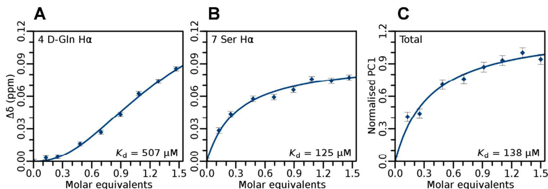
Figure 6. Selected binding isotherms obtained from titrations of geranyl pyrophosphate into Ala 10 -teixobactin demonstrating residue-specific binding behavior with cooperative characteristics. Error bars show RMS of function fit. PC: Principal Component
