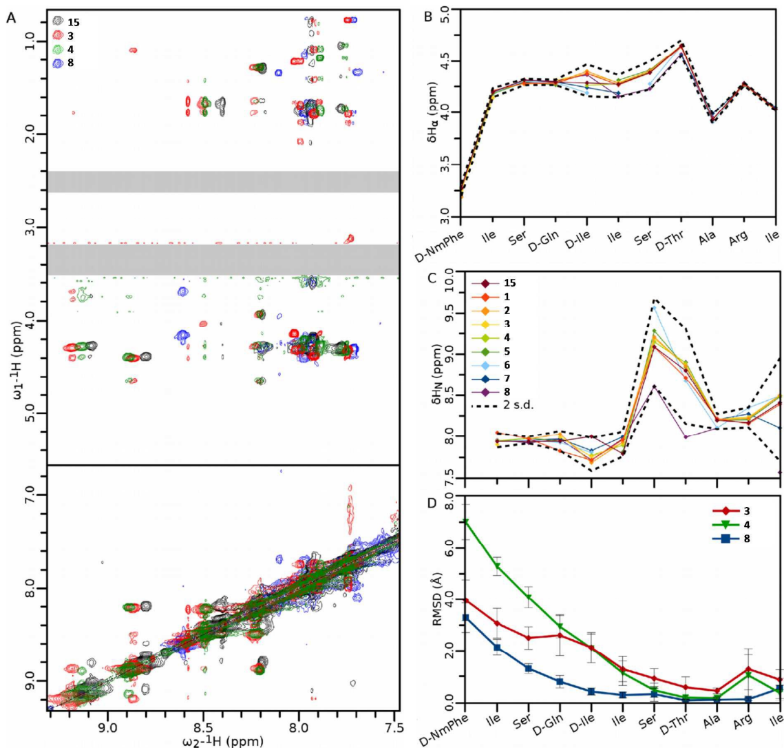
Figure 8. A. Overlay of the amide fingerprint regions of the 1H-1H NOESY spectra of wild type (Arg 10 -teixobactin) and active teixobactin analogues. B and C. Chemical shift data obtained from \alpha (B) and amide (C) protons. D. Statistics of structures calculated using the NOEs obtained from panel A. For clarity, the DMSO (~3.3 ppm) and residual water (~2.5 ppm) signals have been obscured with grey boxes. Data show the average RMSD of each atom in the residue from all 20 members of the ensemble. Error bars are standard deviation in the RMSDs of each residue's atoms. Standard deviations were calculated including the chemical shifts for 15 . 11 Ensembles of 20 structures generated by Cyana 2.1 22 and refined in Gromacs 23 . Error bars indicate standard deviation amongst all the atoms of that residue. Spectra were recorded on 1 mM teixobactin samples dissolved in DMSO- d 6 on a 500 MHz spectrometer at 300 K. Legends for Figure 5B and 5C are the same, and are shown in panel C
