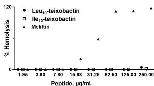
Figure 5. Hemolytic activity of teixobactin analogues 12 and 13 for rabbit erythrocytes. The blood cells were exposed to various concentrations of peptides for 1 h and the release of haemoglobin was determined spectrophotometrically. Each value represents an average of triplicate experiments.
