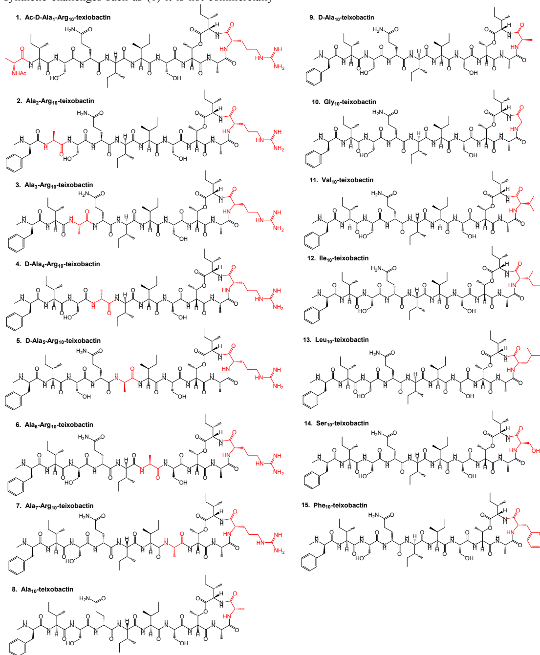
Figure 2. Structure of teixobactin analogues 1-15 synthesised with the replaced amino acids highlighted in red.
