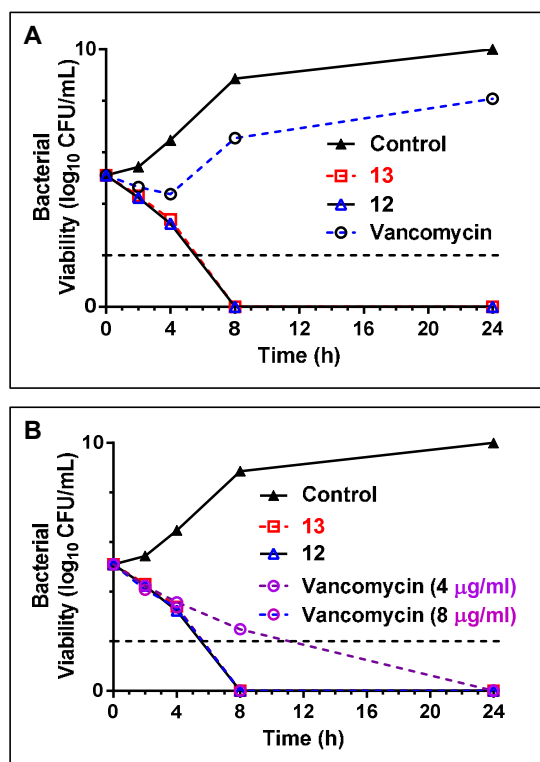
Figure 4. A. Time-kill kinetics of teixobactin analogues 12 & 13 with a comparative antibiotic (vancomycin) against MRSA 21455. The concentration of teixobactin analogues and vancomycin are maintained at 0.5 µg/ml. B. Time-kill kinetics of teixobactin analogues with vancomycin against MRSA 21455 strains at elevated concentrations of the antibiotics. At 8 µg/ml concentration the kill kinetics profiles are similar for vancomycin & teixobactin analogues 12 & 13 . The horizontal dotted line represents the limit of detection.
