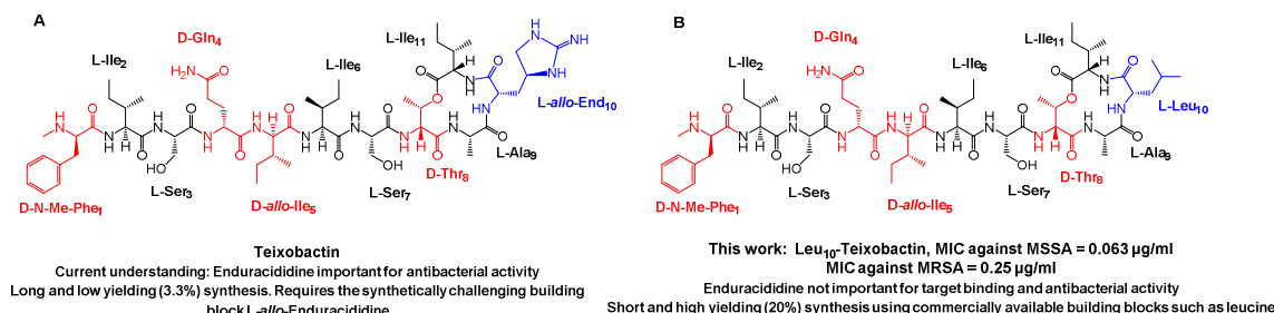
Figure 1. Structure of A. Teixobactin ( 16 ) and B. Leu 10 -Teixobactin ( 13 ) with the D amino acids highlighted in red and the L-allo-End and replaced L-Leu residue highlighted in blue. MRSA ATCC 33591, Staphylococcus aureus ATCC 29213.
