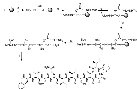
Figure 3. Synthesis of Leu 10 -teixobactin starting from 2-Chlorotritylchloride resin: a. 4 eq. Fmoc-Ala-OH/8 eq. DIPEA in DCM, 3h. b. 20% piperidine in DMF followed by 3 eq. AllocHN-D-Thr-OH, 3 eq. HATU/6 eq. DIPEA, 1.5h. c. 10 eq. Fmoc-Ile-OH, 10 eq. DIC, 5 mol% DMAP in DCM, 2h followed by capping with Ac 2 O/DIPEA 10% in DMF, 20% piperidine in DMF. d. 4 eq. Fmoc-Leu-OH, 4 eq. HATU/8 eq. DIPEA in DMF, 1h followed by 20% piperidine in DMF. e. 10 eq. Trt-Cl, 15% Et 3 N in DCM, 1h. f. 0.2 eq. [Pd(PPh 3 ) 4 ] 0 + 24 eq. PhSiH 3 in dry DCM, 1x20 min, 1x45 min. g. 4 eq. Fmoc/Boc-AA(PG)-OH (AA = amino acid, PG = protecting group), 4 eq. DIC/Oxyrna (μwave, 10 min) followed by 20% piperidine in DMF (3 min, 10 min). h. TFA:TIS:DCM = 2.5:93, 1h. i. 1 eq. HATU/10 eq. DIPEA in DMF, 30 min. j. TFA:TIS:H 2 O = 95:2.5:2.5, 1h.
