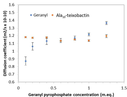
Figure 7. Graph of Diffusion co-efficient vs concentration of geranyl pyrophosphate indicating teixobactin does not aggregate when exposed to increasing geranyl pyrophosphate concentrations. Error bars indicate standard deviation of the fitting function.
