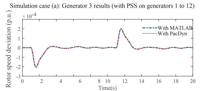
Fig. 16 – 68-bus system: Some simulation results
