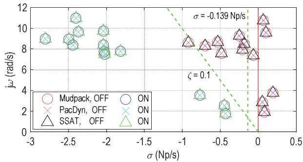
Fig. 13 – 14-generator system, case 2: Comparison of electromechanical modes with PSSs in- (ON) and out-of-service (OFF).
