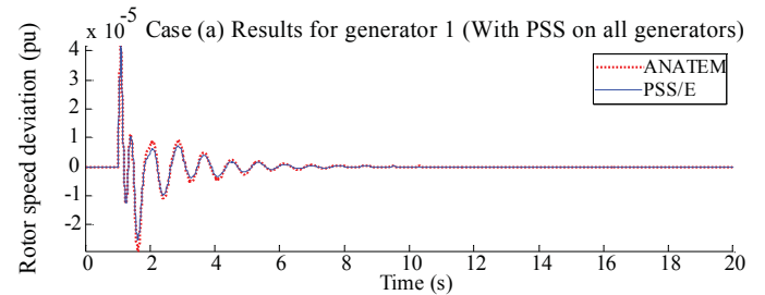
Fig. 8 - 3MIB system: Simulation results for case (a).
