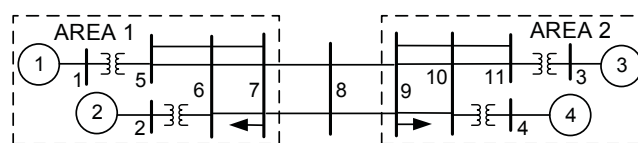
Fig. 3 - Single-line diagram of the 4-generator system
