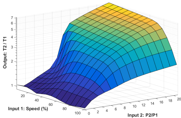
Fig. 6. BNFM 3-D surface plot of inputs (speed and PR) vs. output (TR).
