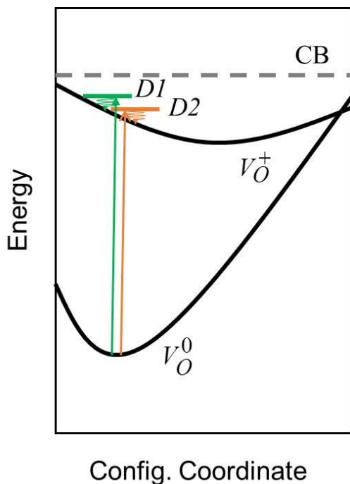
Figure 5. Illustration of proposed model to describe discrete PC transitions. The minimum energy of the oxygen vacancy defect occurs at different values of the lattice configurational coordinate for the V_O^0 and V_O^+ states. The electron is transferred from the V_O^0 state to a nearby ionised donor according to equation 4. Two discrete donors, D1 and D2 , account for the PC peak at 550 and
