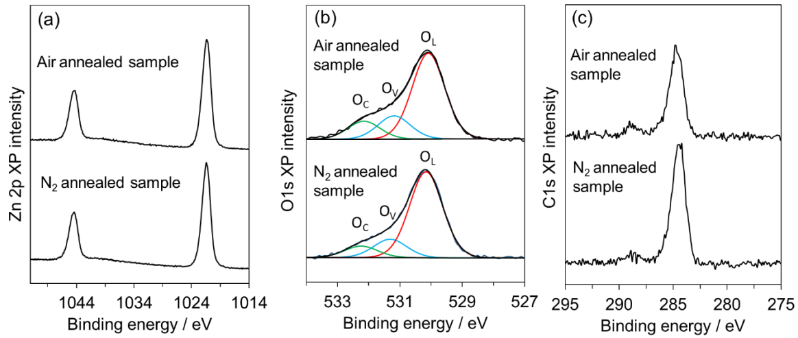
Figure 2. High resolution (a) Zn 2p (b) O 1s and (c) C 1s XPS spectra of ZnO NPs, which were spin-coated prior to annealing either in \text{N}_2 or air at 350 \text{ }^\circ\text{C} .
