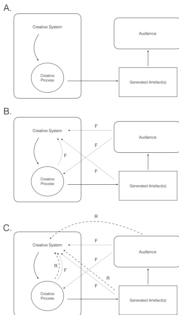
Fig. 1. Illustrating the different aspects of creative systems which may benefit from formal evaluation: The systems range from the merely generative (top), to the fully creative, reflective system (bottom). 1A. The solid lines from the Creative System to the Generated artefact and ultimately to the Audience represent the flow of information through the process of generation without feedback or reflection. 1B. In this system, the dotted lines marked with an 'F' represent feedback from the Audience, or from the Creative Process or Generated artefacts themselves. 1C. This sophisticated type of system incorporates reflection, as denoted by dashed lines marked with an 'R': information regarding the Creative Process, Generated artefacts, and/or the Audience is taken into consideration by the creative system for self-assessment and reflection. It is this last element of reflection that is necessary for qualification as a truly creative system. Note that it is technically possible for a reflective system to not contain feedback, but because this scenario is rare, we focus on the three distinctions illustrated above (purely generative systems, systems containing feedback, and systems containing reflection). Note also that the context in which the Audience and Creative System are embedded is not explicitly shown, but taken to be an implicit part of the Creative System and Audience.
