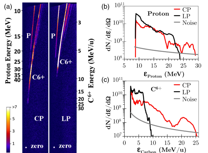
FIG. 2. (a) Raw data from BAS-TR image plates for CP and LP laser pulses irradiating 10-nm amorphous carbon targets. The corresponding CP (red) and LP (black) background-subtracted proton (b) and \text{C}^{6+} spectra (c) with vertical axis units of particles/MeV/sr are also shown. The noise level of +2\sigma is also plotted.
