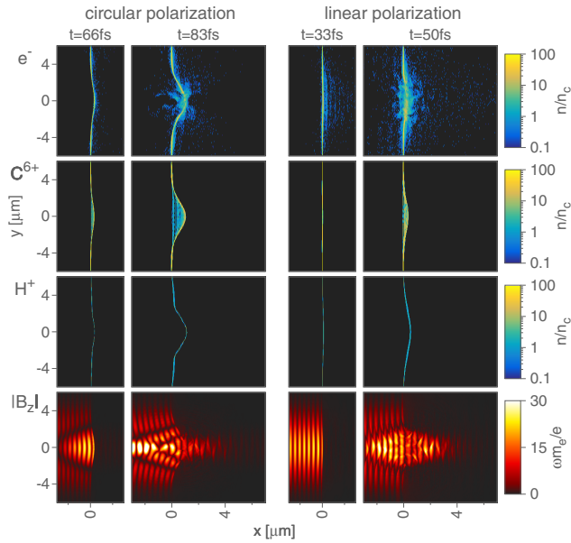
FIG. 4. 3D PIC simulations showing the electron, carbon, and proton densities at different times for both LP and CP. The plot show the density and the magnetic field B_z (corresponding to the laser field for LP) in the plane x - y , which corresponds to the polarization plane for LP.
