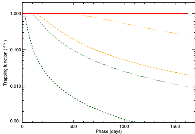
Figure 10. The inferred trapping functions for \gamma -rays ( f^\gamma(t) ) and positrons ( f^+(t) ), from equation (5), resulting from our ‘Case 1’ fits. The green lines correspond to \gamma -rays with t_{56}^\gamma = 35 d (dashed) and t_{57}^\gamma = 160 d (dotted) that we assume for ^{56}\text{Co} and ^{57}\text{Co} decay, respectively. The yellow lines correspond to the leptonic trapping from the ^{56}\text{Co} decay, t_{56}^l = 233 d (dashed), and the leptonic trapping for ^{57}\text{Co} decay, t_{57}^l = 886 d (dotted). The red solid line corresponds to complete trapping.
