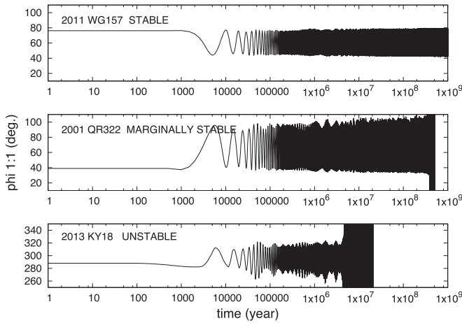
Figure 3. Resonant argument variations of 2011 WG 157 (top), 2001 QR 322 (middle), and 2013 KY 18 (bottom). These represent three types of orbital stability, namely, stable, marginally stable, and unstable NTs, respectively.
