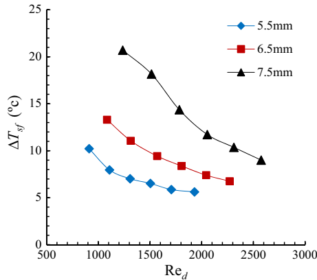
Fig. 7b. Mean temperature difference between the fluid and solid phases versus Re_d number for different spheres diameters and generated heat of Q = 71.52 W.
