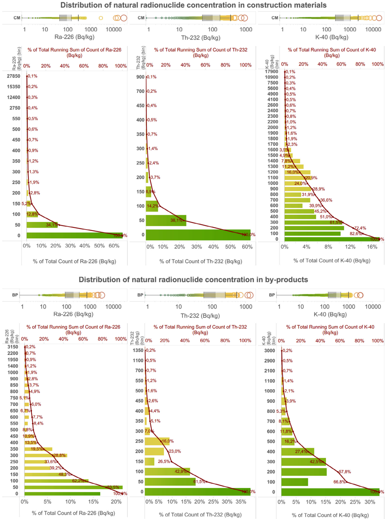
Fig. 2. Distribution of Ra-226, Th-232, and K-40 activity concentration of construction materials and by-products.
