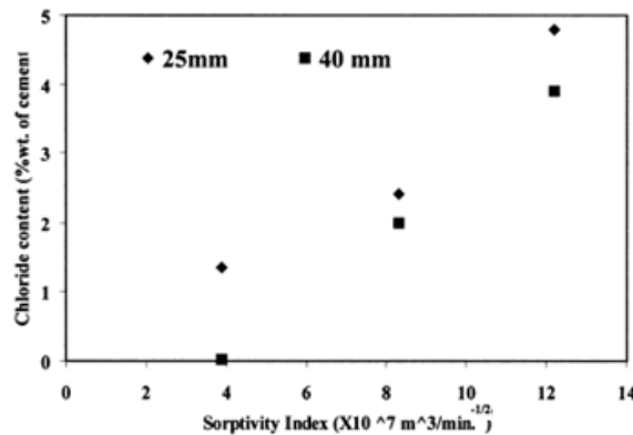
Figure 7: Relationship between sorptivity index and chloride content at two different depths [39]
