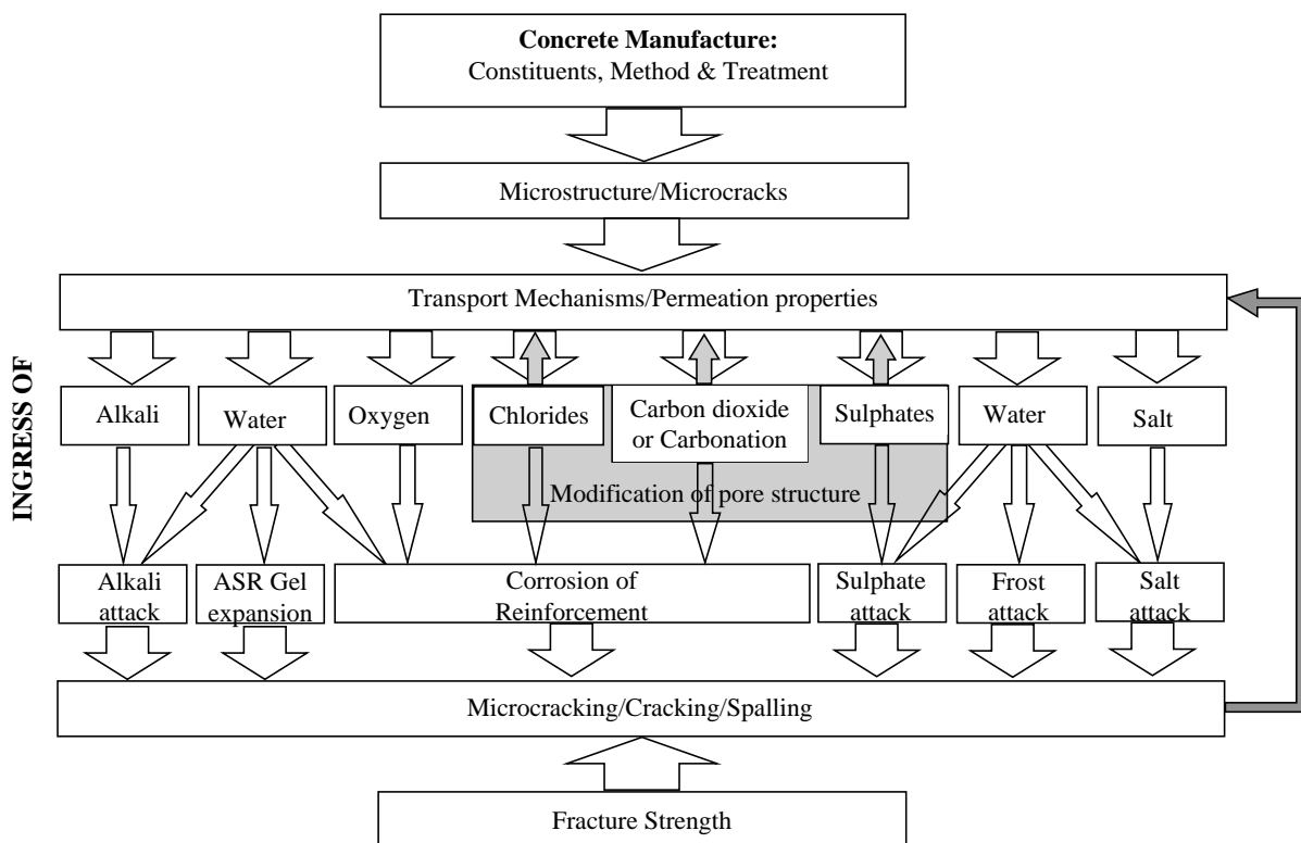
Figure 2: Dependence of durability of concrete on microstructure and transport mechanisms [7]
