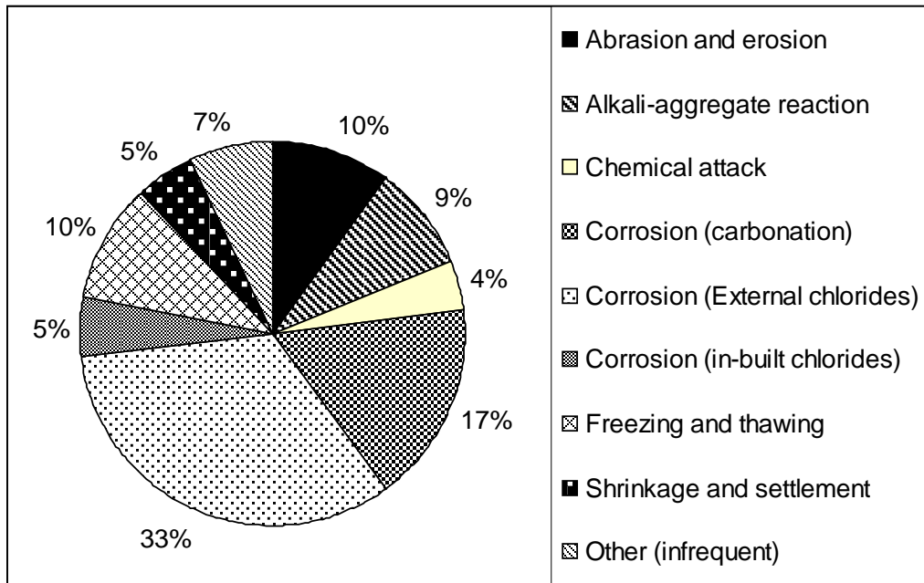
Figure 1: Most frequently reported mechanisms of deterioration of reinforced concrete structures [2]
