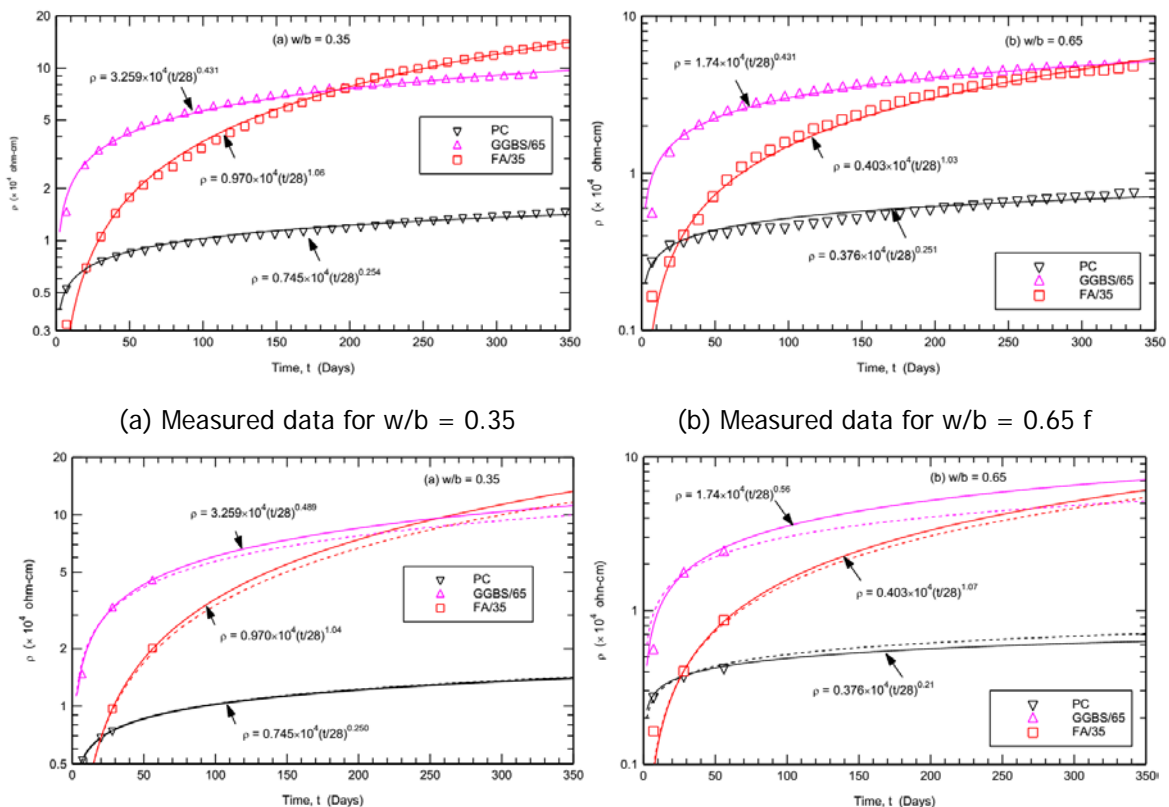
(c) Prediction based on early results for w/b = 0.35 (d) Prediction based on early results for w/b = 0.65 (solid lines in both graphs, Dash lines are curves fitted based on all measurement points)
