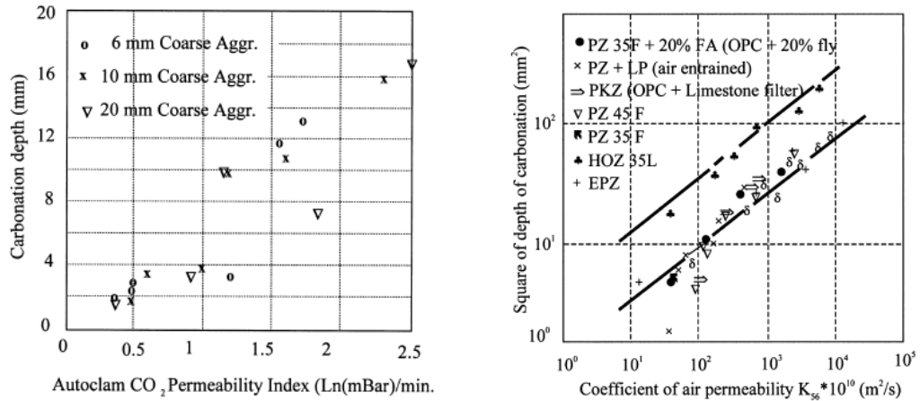
(a) Air (CO 2 ) permeability index (Autoclam) vs carbonation depth [10]
