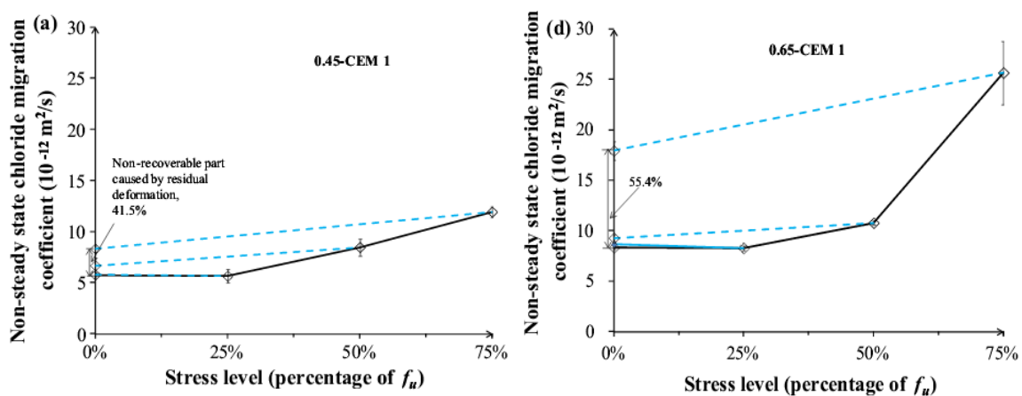
Figure 9: Relationship between applied stress level and chloride migration coefficient [40]
