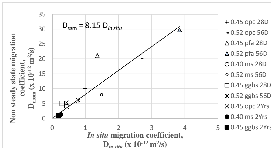
Figure 5: Correlation between Permit in situ migration coefficient and non-steady state migration coefficient for different types of concrete [34]
