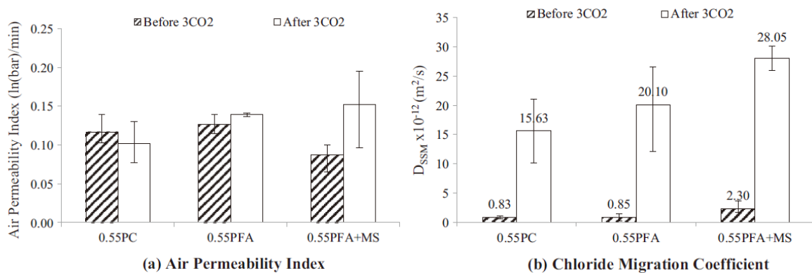
Figure 10: Influence of carbonation on air permeability and chloride migration coefficient of different types of concrete [41]
