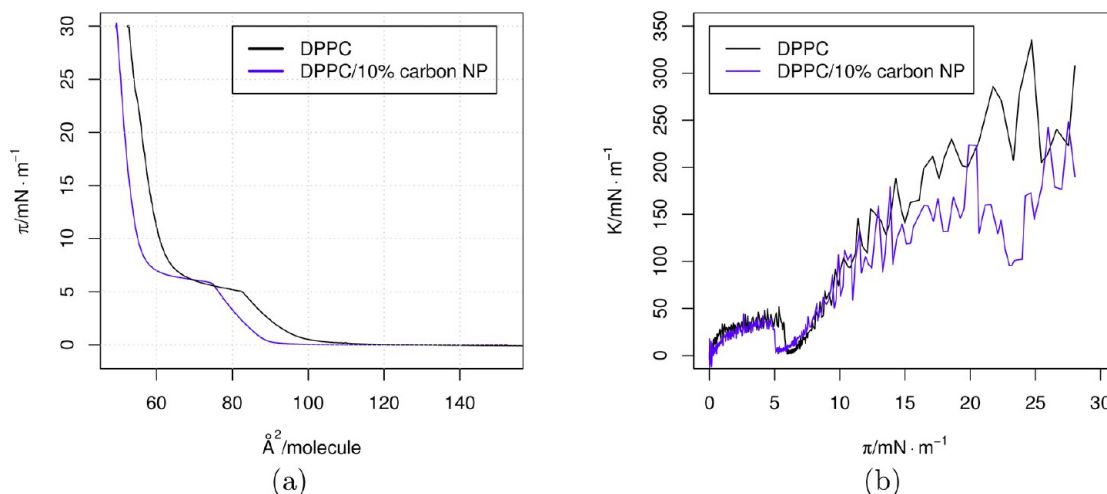
Figure 3. Surface pressure–area isotherms (a) and compression modulus plots (b) for DPPC monolayers as measured on a Langmuir–Blodgett trough. Isotherms were measured for pure DPPC and DPPC including 10.0% carbon nanoparticles to DPPC by mass. Isotherms were measured at 20 \pm 1 °C.
