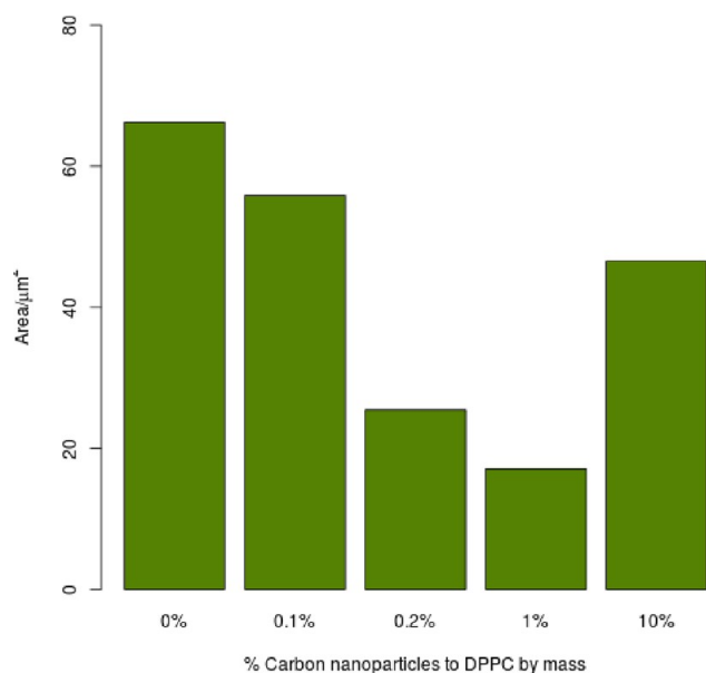
Figure 10. Plot of average sizes of DPPC domains on aqueous subphase as measured by BAM at 8.3 \text{ mN m}^{-1} . The domain sizes were measured for DPPC with various concentrations of carbon nanoparticles. The average domain sizes for the concentrations of carbon nanoparticles were 66.2 \mu\text{m}^2 (0%), 55.9 \mu\text{m}^2 (0.1%), 25.5 \mu\text{m}^2 (0.2%), 17.1 \mu\text{m}^2 (1%), and 46.6 \mu\text{m}^2 (10%).
