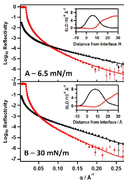
Figure 11. Neutron reflectivity of monolayers of pure DPPC (open diamonds) and DPPC with 10% by mass carbon nanoparticles (filled circles). The surface pressure was held at (A) 6.5 \text{ mN m}^{-1} and (B) 30 \text{ mN m}^{-1} during the measurements. The black data points are from d62-DPPC on a subphase of null reflecting water, and the red data points are from h62-DPPC on a subphase of \text{D}_2\text{O} .
