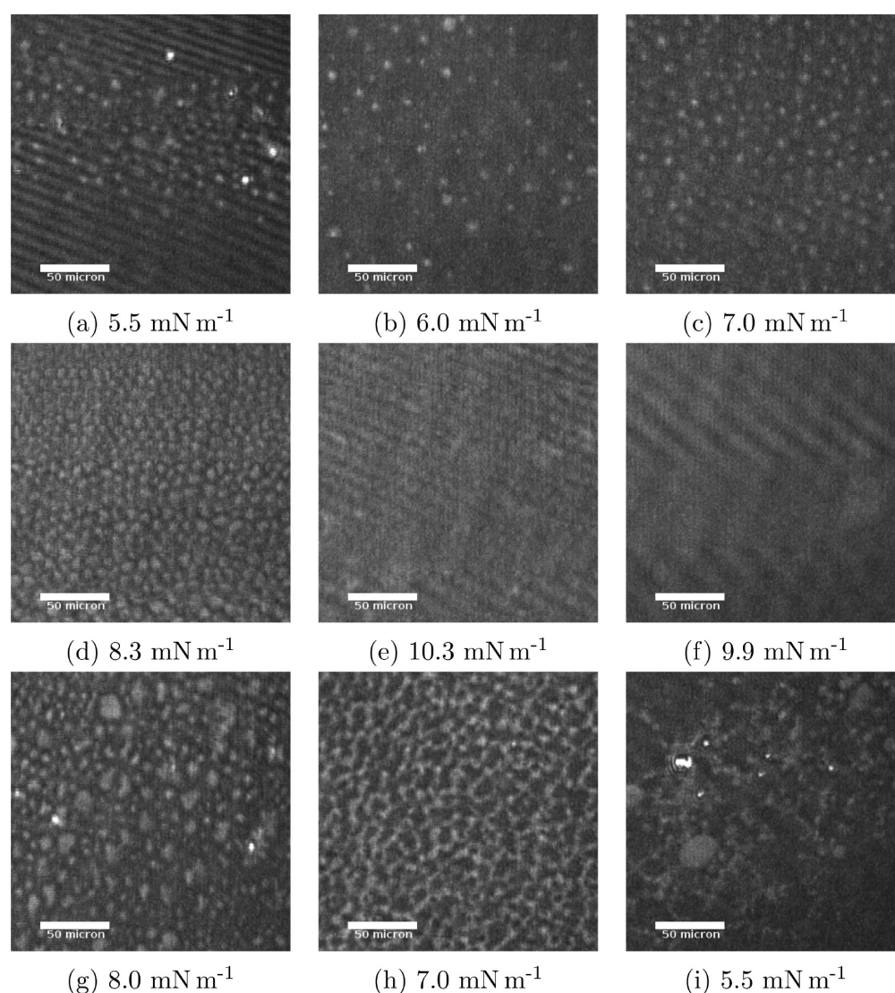
Figure 8. BAM images of 1.0% carbon nanoparticles to DPPC by mass on aqueous subphase. Images show liquid-condensed domains as surface pressure is increased from 5.5 \text{ mN m}^{-1} by compression of the monolayer to a maximum of 10.3 \text{ mN m}^{-1} , before expanding the monolayer again to a surface pressure of 5.5 \text{ mN m}^{-1} . With the presence of the nanoparticles, the domains are smaller and more numerous than the domains observed with DPPC alone. During expansion, the lipid forms irregular, stringlike domains, and no reoccurrence of the large, round domains as seen with pure DPPC is observed.
