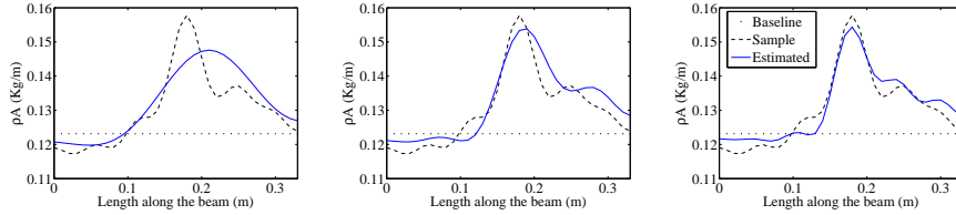
Figure 11: Baseline, sample and reconstructed random field sample of the mass along the length using 4 (LHS), 8 (middle) and 12 (RHS) modes.
