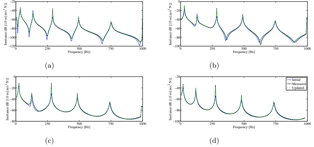
Figure 7: Comparison between an initial value, updated and the synthetic measured using four FRFs (a) at 0 * L , (b) 0.25 * L , (c) 0.70 * L , and (d) L .
