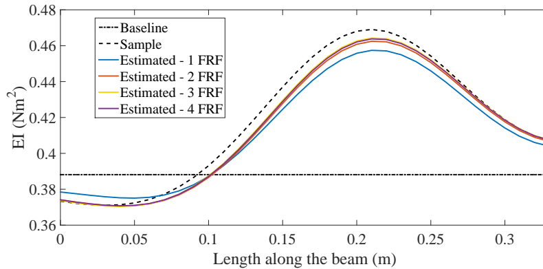
Figure 2: Baseline, sample and reconstructed random field sample of the flexural rigidity along the length using 1,2,3, and 4 FRFs in the estimation.
