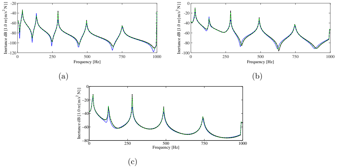
Figure 6: Comparison between an initial value, updated and the synthetic measured using three FRFs (a) at 0 * L , (b) at 0.25 * L , and (c) at 0.70 * L .
