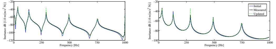
Figure 12: Comparison among an initial, updated and the synthetic measured FRF at node 1 (LHS) and node 2 (RHS). Updated FRFs calculated with the random field sample reconstructed with 4 modes.
