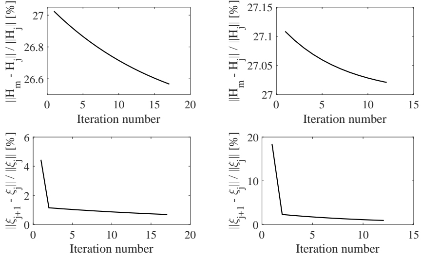
Figure 23: Convergence of the FRF ( \|\mathbf{H}_m - \mathbf{H}_j\| ) and parameters ( \|\xi_{j+1} - \xi_j\| ) using 4 (LHS) and 6 (RHS) terms in the KL expansion.
