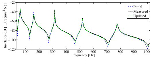
Figure 4: Comparison between the FRF obtained with an initial value, and updated value, and the synthetic measured FRF using one FRF at node 1( 0 * L ).
