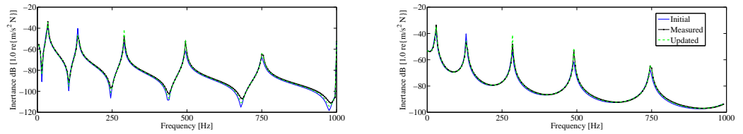
Figure 14: Comparison among an initial, updated and the measured FRF at node 1 (LHS) and node 2 (RHS). Updated FRFs calculated with the random field sample reconstructed with 12 modes.
