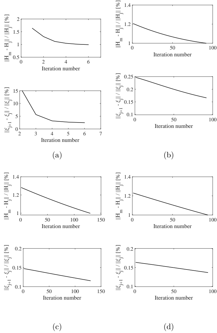
Figure 9: Convergence of the FRF residual ( \|\mathbf{H}_m - \mathbf{H}_j\| ) and parameters ( \|\xi_{j+1} - \xi_j\| ) using (a) 1 FRF, (b) 2 FRFs, (c) 3 FRFs, and (d) 4 FRFs.
