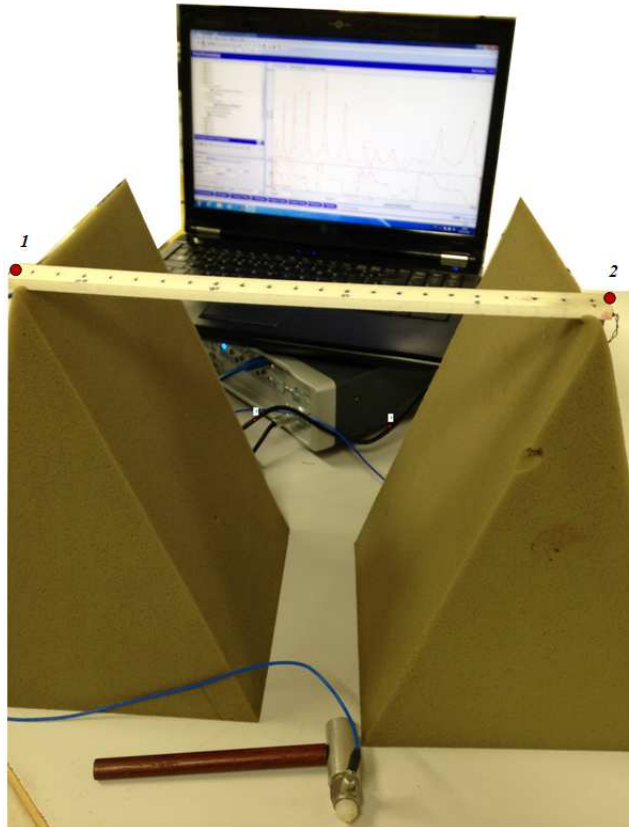
Figure 18: The test rig for the free-free beam.
