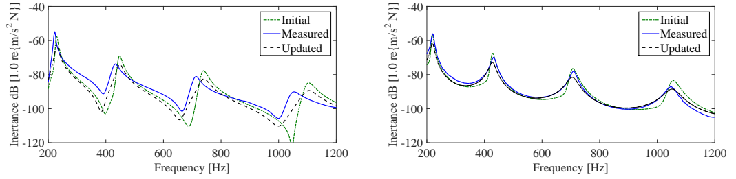
Figure 20: Comparison between an initial value, updated and the experimental measured FRF at node 1 (LHS) and at node 2 (RHS) using 4 terms in the KL expansion.
