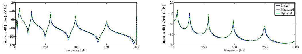
Figure 13: Comparison among an initial, updated and the synthetic measured FRF at node 1 (LHS) and node 2 (RHS). Updated FRFs calculated with the random field sample reconstructed with 8 modes.
