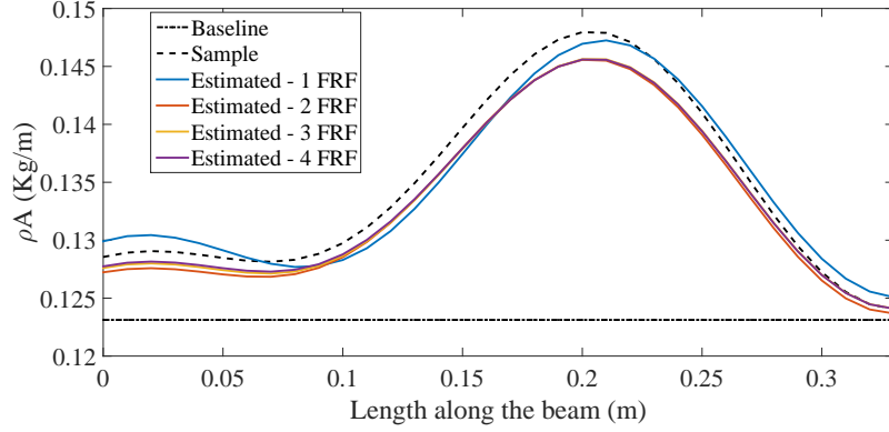
Figure 3: Baseline, sample and reconstructed random field sample of the mass per unit of length using 1,2,3, and 4 FRFs in the estimation.
