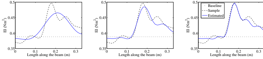
Figure 10: Baseline, sample and reconstructed random field sample of the flexural rigidity along the length using 4 (LHS), 8 (middle) and 12 (RHS) modes.
