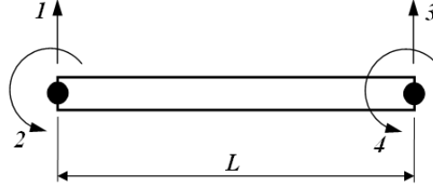
Figure 1: Two-node beam spectral element
