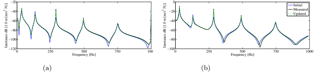
Figure 5: Comparison between an initial value, updated and the synthetic measured using two FRFs (a) at 0 * L and (b) at 0.25 * L .
