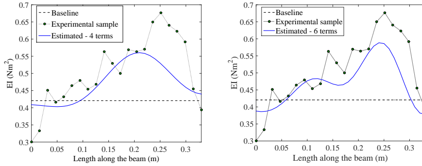
Figure 19: Baseline, experiential sample and reconstructed random field sample of the flexural rigidity ( EI(x) ) with 4 (LHS) and 6 (RHS) terms in the KL expansion.
