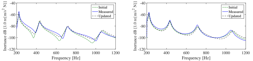
Figure 21: Comparison between an initial value, updated and the experimental measured FRF at node 1 (LHS) and at node 2 (RHS) using 6 terms in the KL expansion.
