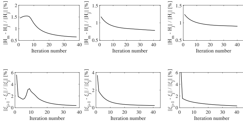
Figure 16: Convergence of the FRF ( \|\mathbf{H}_m - \mathbf{H}_j\| ) and parameters ( \|\xi_{j+1} - \xi_j\| ) using 4 (LHS), 8 (middle) and 12 (RHS) terms in the KL expansion.
