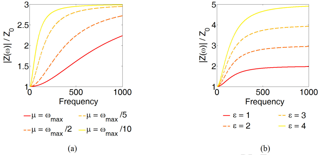
Figure 10: (a) Effect of variation of \mu on the viscoelastic modulus of regular hexagonal lattices (considering a constant value of \epsilon = 2 ) (b) Effect of variation of \epsilon on the viscoelastic modulus of regular hexagonal lattices (considering a constant value of \mu = \omega_{\max}/5 ). Here Z represents the viscoelastic moduli (i.e. E_1 , E_2 and G_{12} ) and Z_0 is the corresponding elastic modulus value for \omega = 0 .
