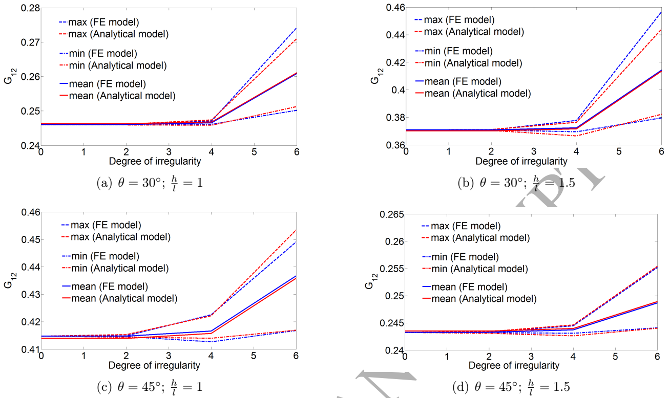
Figure 5: Effective shear modulus ( G_{12} ) of irregular lattices with different structural configurations considering correlated attributes
