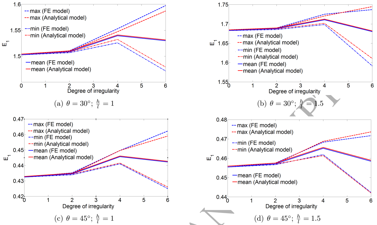
Figure 3: Effective Young's modulus ( E_1 ) of irregular lattices with different structural configurations considering correlated attributes
