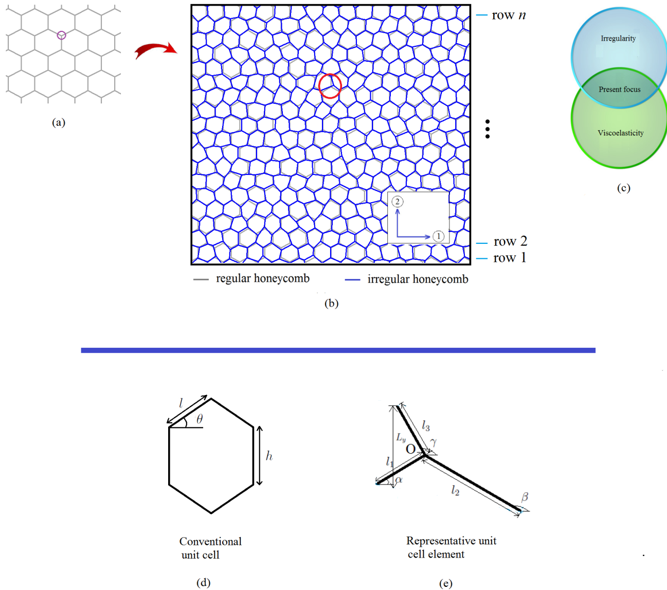
Figure 1: (a) Illustration to define degree of irregularity and perturbation of nodes (b) Typical representation of irregular honeycomb (c) Scope and focus of the present study (d) Conventional unit cell for regular lattices (e) Representative unit cell element (RUCE) for the analysis of spatially irregular lattices
