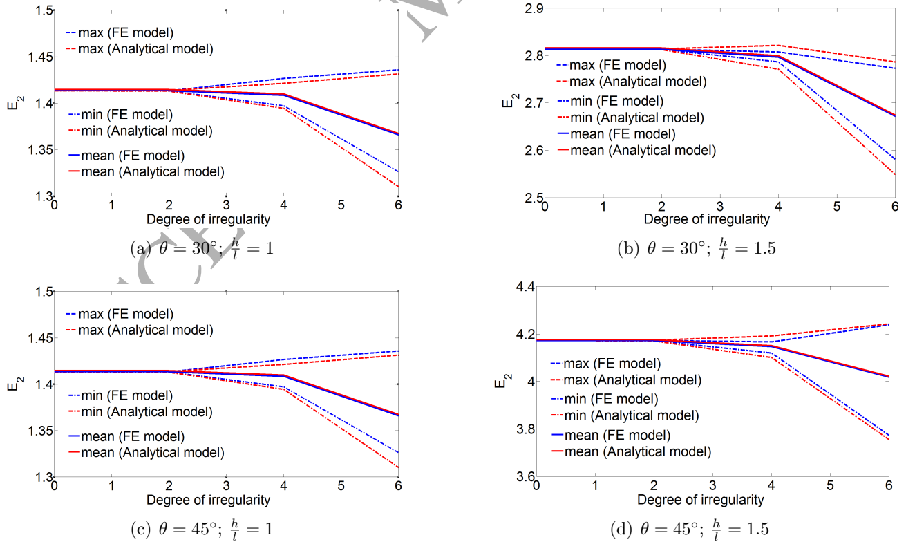
Figure 4: Effective Young's modulus ( E_2 ) of irregular lattices with different structural configurations considering correlated attributes
