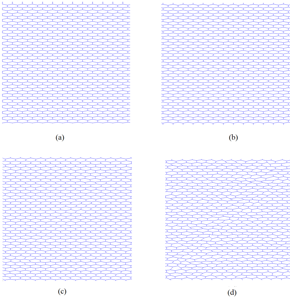
Figure 13: Structural configurations for a single random realization of an irregular hexagonal lattice considering deterministic cell angle \theta = 30^\circ and h/l = 1 : (a) r = 0 (b) r = 2 (c) r = 4 (d) r = 6
