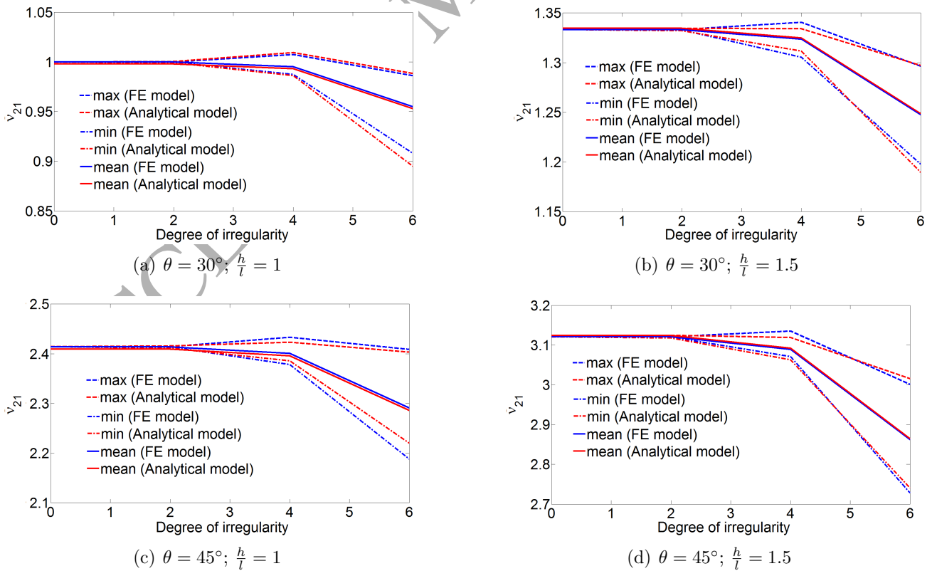
Figure 7: Effective Poisson's ratio ( \nu_{21} ) of irregular lattices with different structural configurations considering correlated attributes
