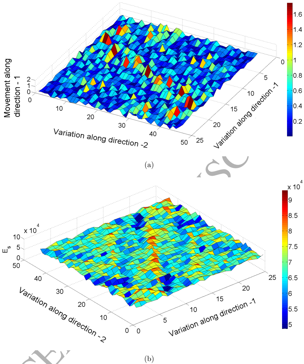
Figure 12: Typical representation of random fields for a particular realization considered in the analysis for (a) movement of the top vertices of a tessellating hexagonal unit cell with respect to the corresponding deterministic locations ( r = 6 ) (b) intrinsic elastic modulus ( E_s ) with \Delta_m = 0.002
