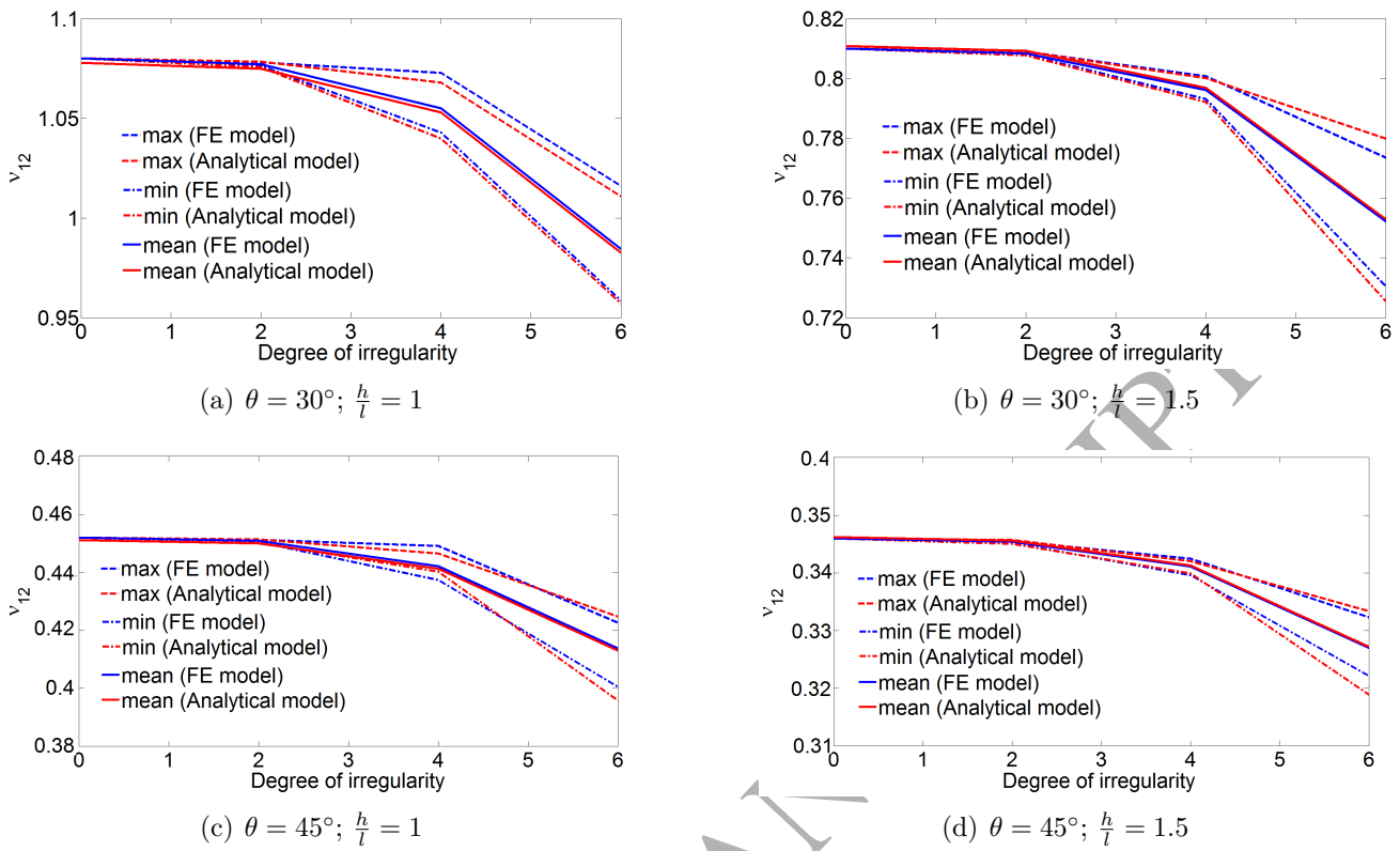
Figure 6: Effective Poisson's ratio ( \nu_{12} ) of irregular lattices with different structural configurations considering correlated attributes
