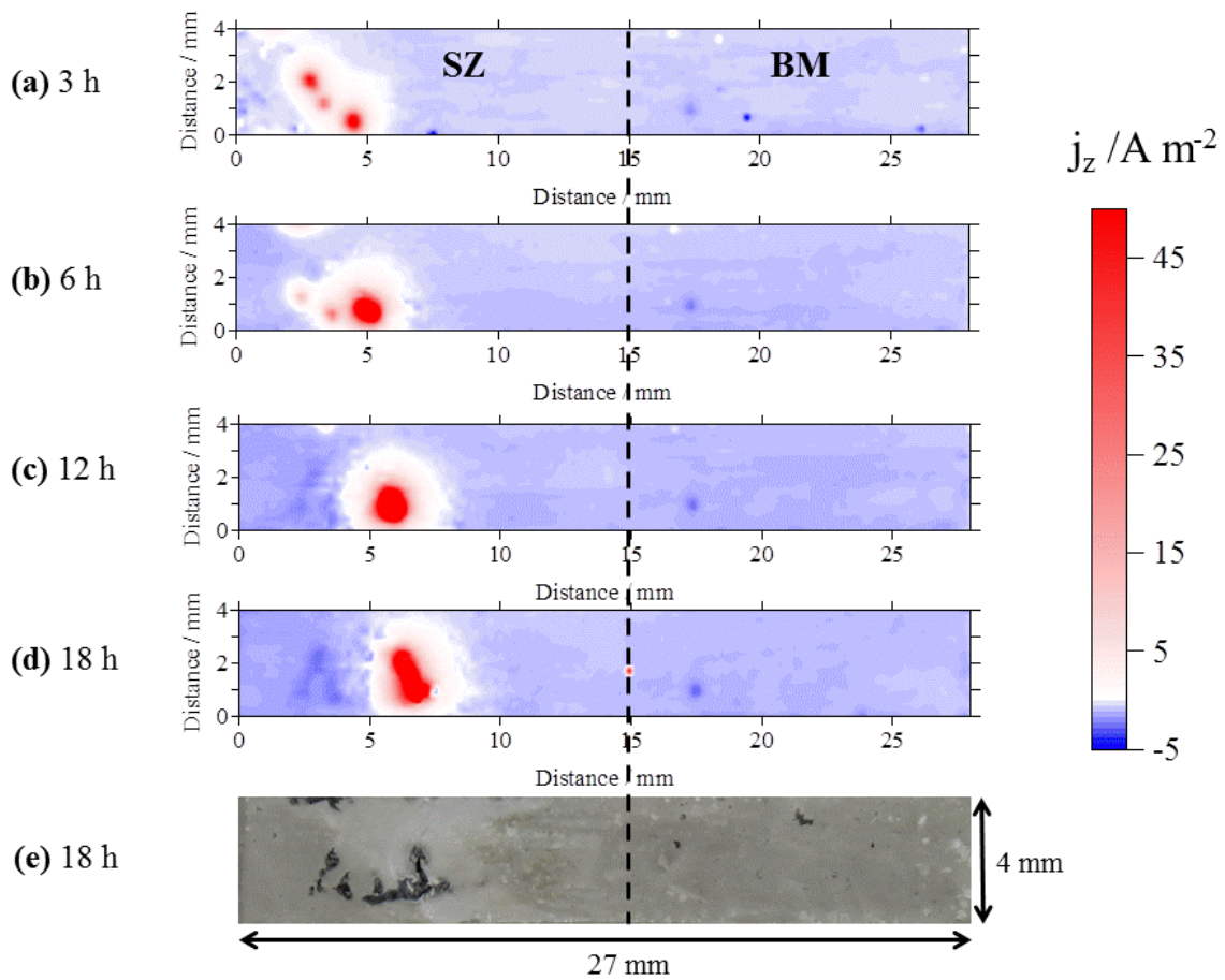
Fig. 4. (a-d) Series of SVET-derived j_z distribution maps recorded from the surface of the welded joint sample over an 18 h immersion in a 5 wt.% NaCl (aq) electrolyte, (e) along with a photographic image of the post-corrosion surface.
