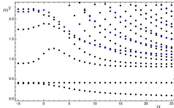
FIG. 2: The mass spectrum m^2 of scalar (black) and tensor (blue) states.
