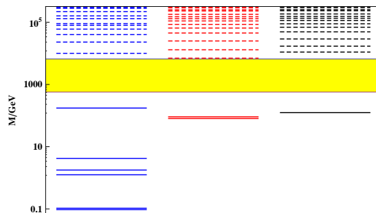
FIG. 1: The mass spectrum of SM particles (continuous lines) and of a generic strongly-coupled new theory (dashed lines) with new states heavy enough to evade the bounds from LHC direct searches (shaded region) [2, 3]. Fermions are rendered in blue, vectors in red and scalars in black.
