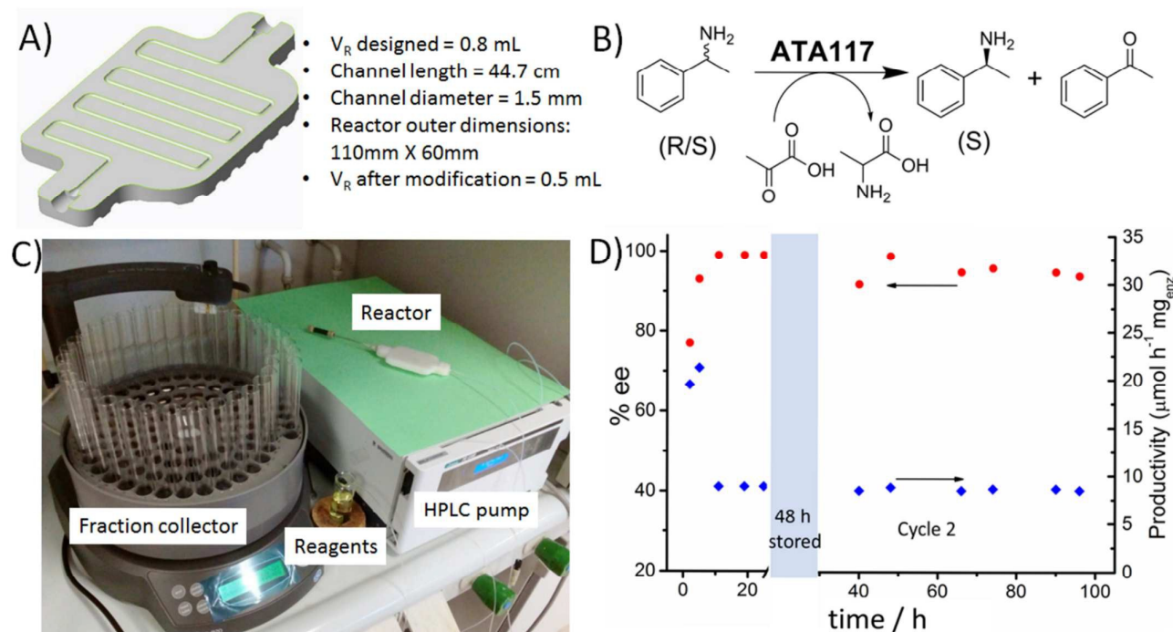
Figure 5. Continuous-flow biocatalytic reactors for the kinetic resolution of rac -methylbenzylamine employing ATA 117 supported on the 3D printed bioreactor. A) CAD of the bioreactor and main reactor parameters. B) Kinetic resolution of rac -methylbenzylamine employing ATA 117 supported on the 3D printed bioreactor. C) Experimental set-up employed for the continuous-flow biocatalytic transformation. D) Productivity and enantiomeric excess observed as a function of time. The first two data points correspond to experiments assayed at 25 \mu\text{L}\cdot\text{min}^{-1} , while the rest were assayed at 10 \mu\text{L}\cdot\text{min}^{-1} . The plot represents two separate runs under continuous-flow, the first of them for 24 h, followed by a 48 h storage in fresh buffer and a subsequent run for further 78 h. The results indicate the activity and stability of the enzyme, by keeping its activity over extended periods of time (ca. 100 h) under continuous-flow streams.
