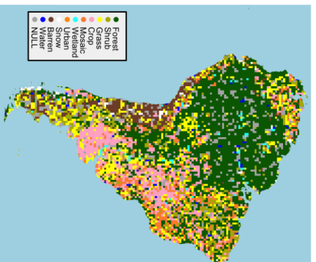
Possibility
