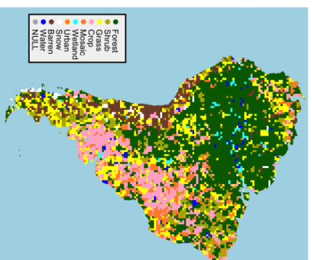
Bayesian Prob
