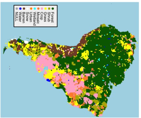
Bayesian Prob
