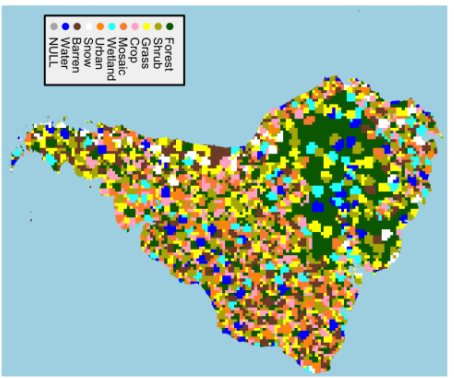
Fuzzy Sets
