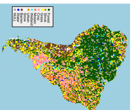
Fuzzy Sets
