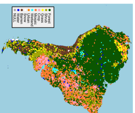
Reference Data
