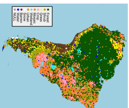
Reference Data
