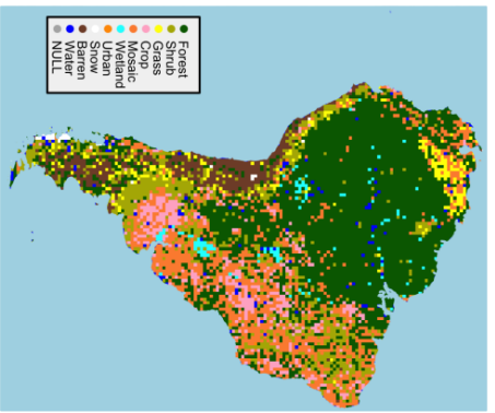
Reference Data
