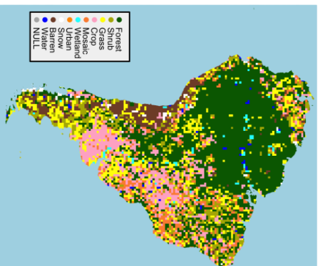
Possibility
