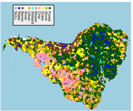
Dempster-Shafer
