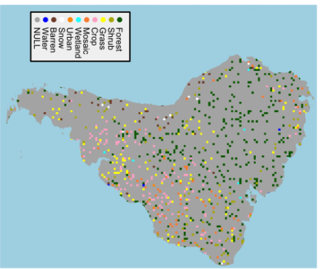
Possibility
