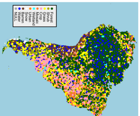
Dempster-Shafer
