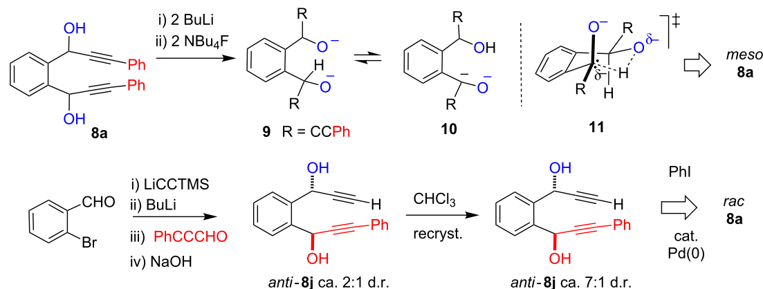
Scheme 3: Equilibration to meso species.
