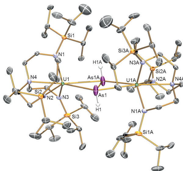
Figure 1. Molecular structure of 3 at 120 K with ellipsoids set at 50% probability. [31] Non-arsenic-bound hydrogen atoms are omitted for clarity. An arbitrary pair of \text{HAsAsH} hydride positions corresponding to an E isomer have been selected, with the other pair omitted for clarity. Selected distances [Å]: U1–As1 3.1203(7), U1–As1A 3.1273(7), U1–N1 2.256(4), U1–N2 2.273(4), U1–N3 2.261(4), U1–N4 2.709(4), As1–As1A 2.4102(13).
