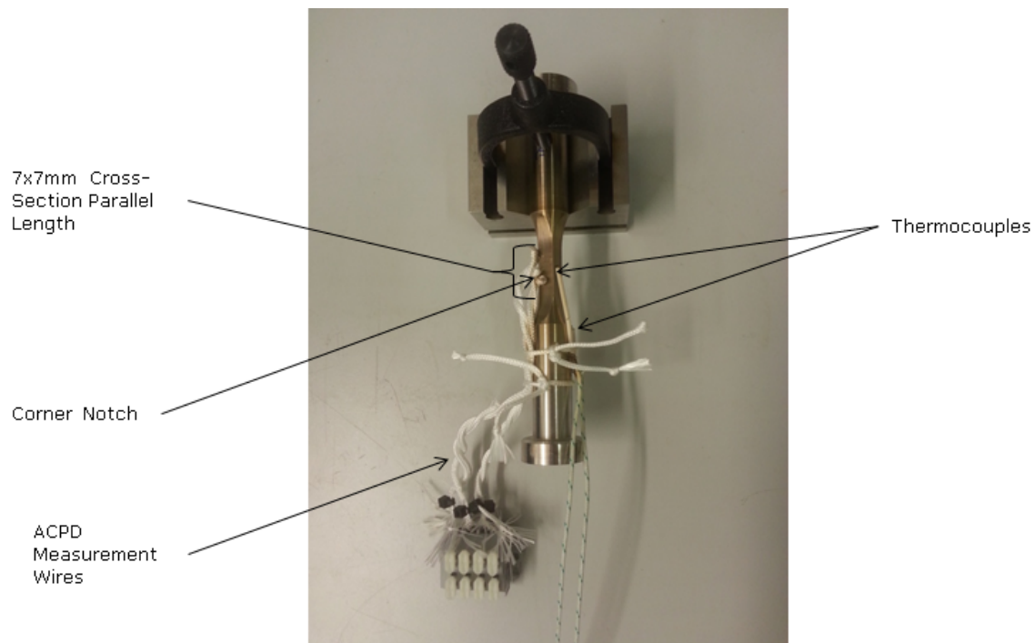
Figure 1 – Instrumented Sample
