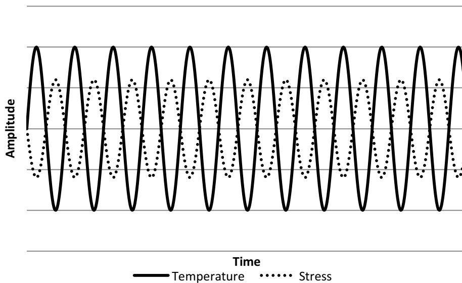
Figure 4 – OP TMF
