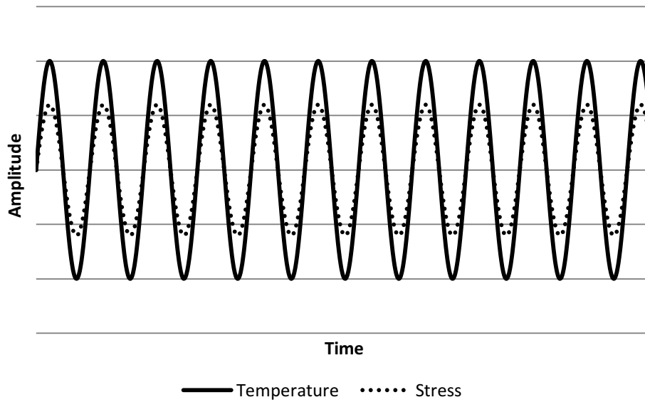
Figure 3 – IP TMF
