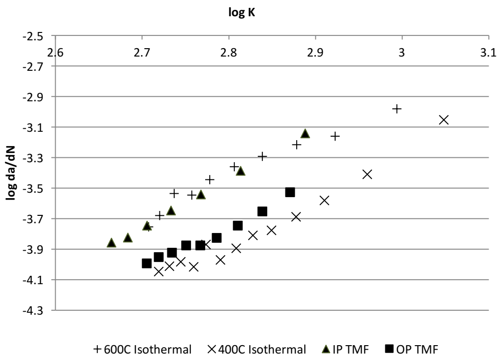
Figure 5 – Crack Growth Rates
