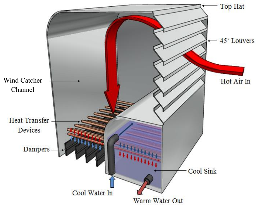
Figure 2 Cooling wind catcher with heat pipes.
