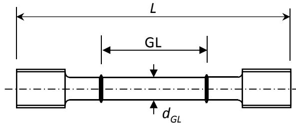
Figure 2: "Standard" uniaxial creep test specimen ( GL \approx 30 - 50\text{mm} ; d_{GL} \approx 6 - 10\text{mm} ; L \approx 100 - 130\text{mm} ).
