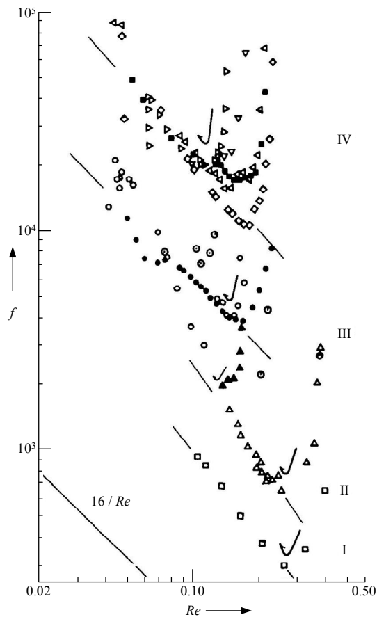
Fig. 6 Friction factor f versus Reynolds number for water flow in xylem [35] .
