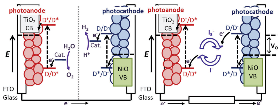
Fig. 1 Schematic energy level diagram of a photoelectrosynthesis cell for splitting H 2 O (left) and a tandem DSC where a n-type photoanode and a p-type photocathode are incorporated into one device (right).
