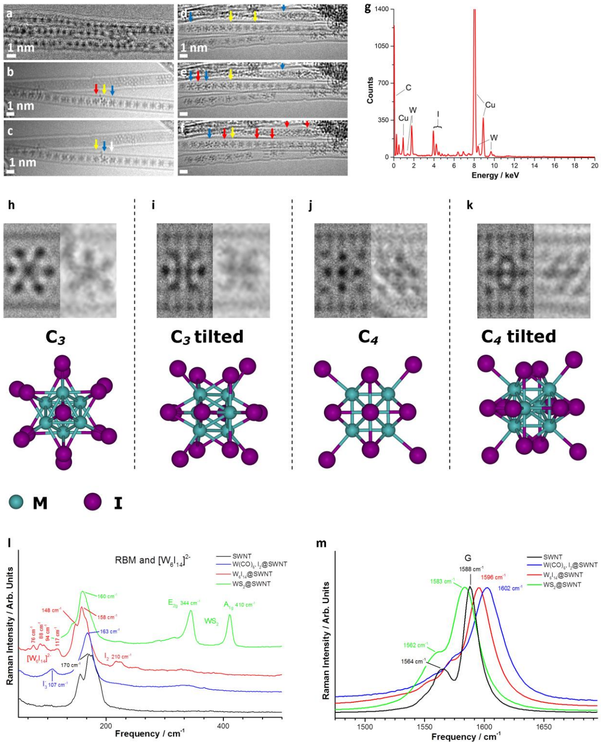
Figure 2. (a) 100 kV HRTEM and (b-f) 80kV AC-HRTEM images of n\text{-}[\text{W}_6\text{I}_{14}]^{2-}\text{@SWNT}^{2n+} demonstrating the tumbling motion of metal clusters over time (marked by arrows). (g) The EDX spectrum confirms the elemental composition of the clusters. Please note that the Cu peaks are due to the TEM specimen grid. (h-k) High magnification images of the four principal projections of octahedral [\text{W}_6\text{I}_{14}]^{2-} and their corresponding atomic models. (l) Raman spectra in the low-frequency region showing the bands of the products formed inside the nanotubes at each stage of the multi-step synthesis (polyiodide chains – blue; [\text{W}_6\text{I}_{14}]^{2-} nanoclusters – red; [\text{WS}_2]_n nanoribbons – green), and (m) a strong blue shift of the Raman G-band of SWNT indicative of the positive charge on SWNT due to the electron transfer to the guest-species polyiodide chains – blue or metal iodide nanoclusters –
