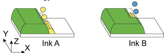
Fig. 2 Process of FRIJP showing line print in the Y direction, with number of lines increasing in the X direction. Each ink is printed in series, first ink A (yellow), then ink B (blue) only when both inks are printed can the curing occur (green). Layers are counted in total reacted (green) layers printed.
