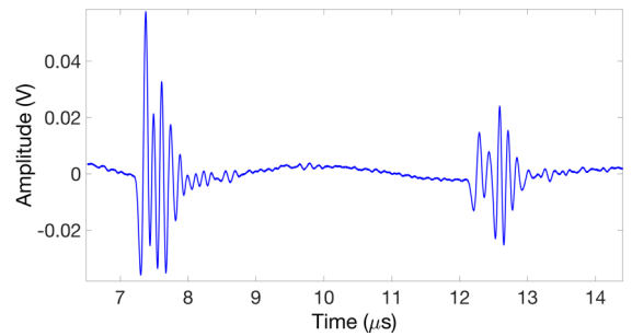
Fig. 6. The pulse echoes with 10 MHz center frequencies from reflections at the bottom left of back wall of a corroded sample after 303 mins of corrosion.
