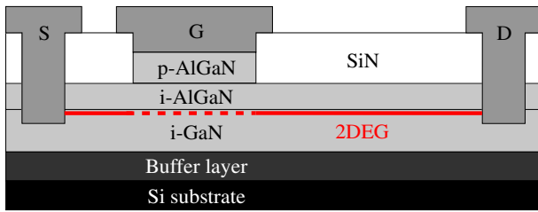
Fig. 1. Simplified cross-section of the investigated transistor. The gate prevents a p-doped AlGaIn layer for the enhancement-mode operation.
