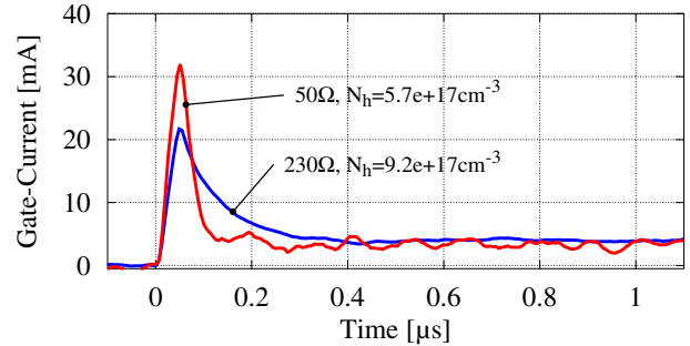
Fig. 13. Experimental waveforms of the bias-conditions for a similar operation-point, comparing condition C in two different optimisations.
