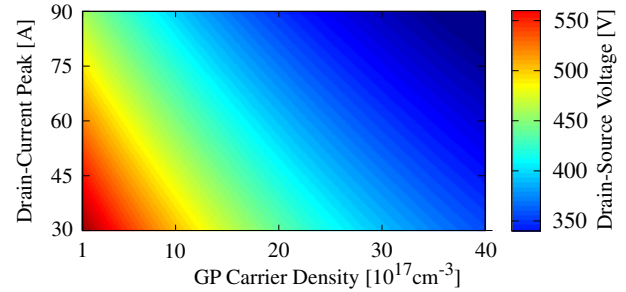
Fig. 9. Short-circuit safe operating area (SCSOA) of p-gate HEMTs. Achievable drain-source voltage in the respective condition of the drain-current peak and the gate-current peak (GP) related carrier density.
