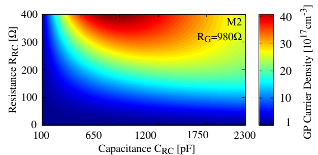
Fig. 10. Simulated result of the originated gate-current peak (GP) related carrier density. The density can be adjusted regarding the parametrisation of the modulation-network branch containing R_{RC} and C_{RC} .
