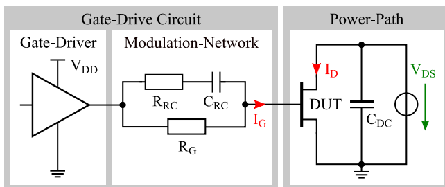
Fig. 2. Test set-up, composed of: a galvanic (optical) decoupled gate-driver, a modulation-network of the gate-signal (typ. GaN app.), and a power-path with the device under test (DUT).
