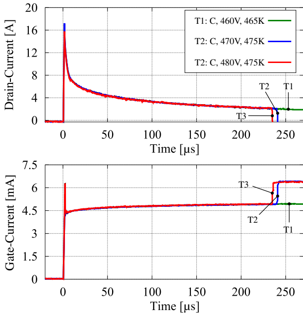
Fig. 7. Experimental results of the thermal failure mode, comparing condition C in a variation of power dissipation and ambient-temperature.
