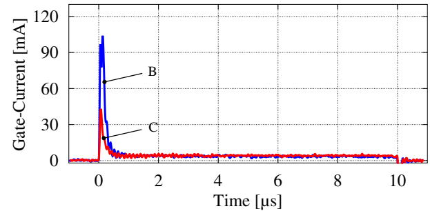
Fig. 6. Experimental waveforms of the bias-conditions for a similar operation-point, comparing condition B and C.
