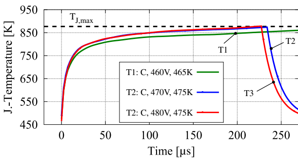
Fig. 8. Simulated results of the respective junction-temperature according to the thermal-failure mode, presented in Fig. 7. The estimate is conducted with usage of a numerical 3D temperature simulator.
