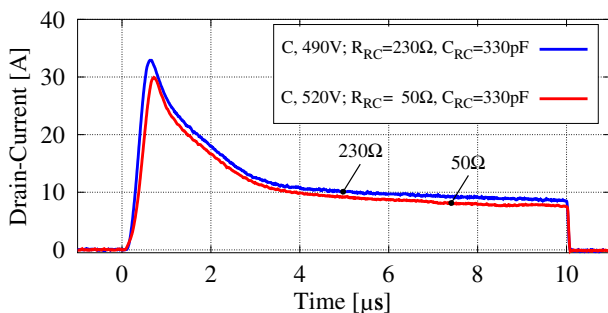
Fig. 12. Experimental results of maximum voltage withstand capability, comparing condition C in two different optimisations before failure.
