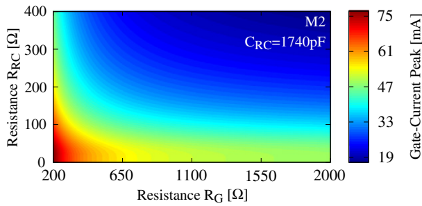
Fig. 11. Simulated result of the originated gate-current peak value. The value can be adjusted regarding the parametrisation of the modulation-network resistance R_G and R_{RC} .
