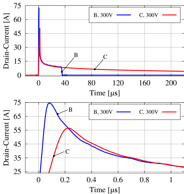
Fig. 5. Experimental results of maximum time withstand capability, comparing the conditions B and C before failure. Although an equivalent peak of condition A, due to the gathered observations in Section 3.1, the capability is less than B.
