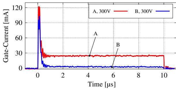
Fig. 4. Experimental waveforms of the bias-conditions for a similar operation point, comparing conditions A and B. The waveforms of the gate-source voltages are approximately identical.
