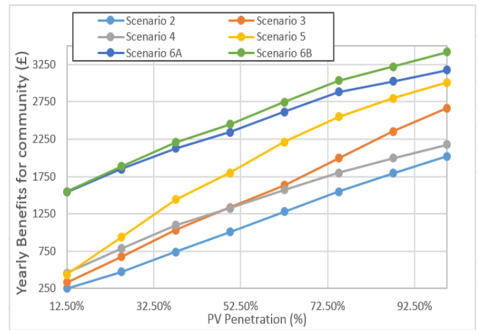
Fig. 13. Yearly community benefits for all scenarios (CES capacity: 96kWh)
