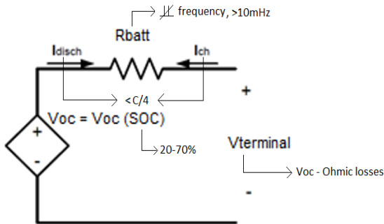
Fig. 6. Equivalent battery electric-circuit used
