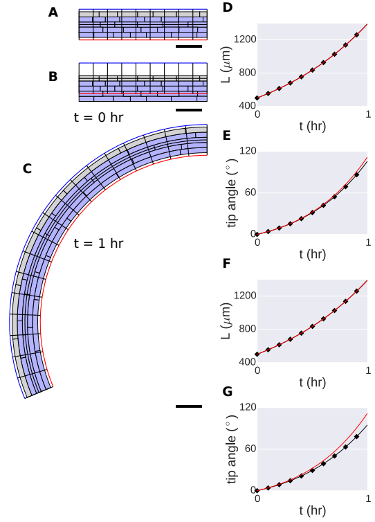
Figure 4: Bending through differences in cell-wall viscosity. (a) Initial artificial geometry with five files of cells. The uppermost file has (gray) lower viscosity ( \mu = 0.13 ) relative to the other cells (blue, \mu = 0.15 ). The discretized midline is overlaid with black lines between red and blue boundaries indicating cross-sectional orientations. (b) Same geometry as (a) but with midline offset from centre of the organ. (c) Simulation at t = 1 hr. Length (d) and tip angle (e), with midline at the organ centre (red) or offset (black with diamonds). (f,g) Comparison of midline (red) and vertex-element (black with diamonds) simulations (based on [17]). Scale bar 100 \mu\text{m} .
