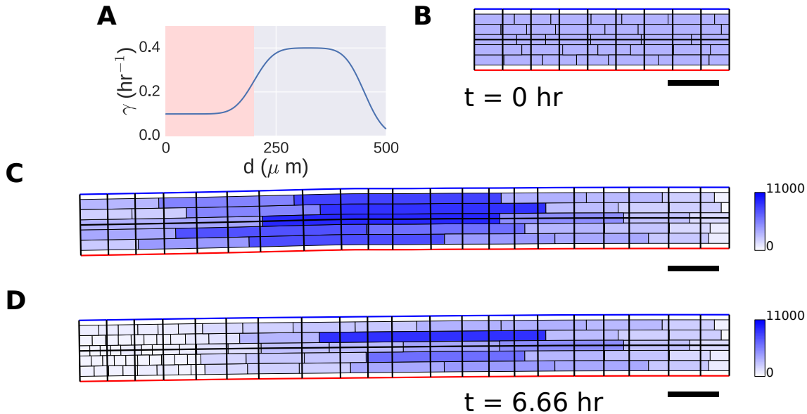
Figure 6: Simulations with axial variation in cell-wall properties. (a) Elongation rate \gamma as a function of the distance d = L - s from the organ tip. (b) Initial artificial geometry (as in Figure 4). The organ is anchored ( s = 0, d = L ) at its right-hand end, and the tip of the organ ( s = L, d = 0 ) is at the left. (c) Simulation at t = 6.66 hr. (d) Simulation with cell-division (within the pink region of (a)). Colour bars indicate cell areas ( \mu\text{m}^2 ). Scale bar 100 \mu\text{m} .
