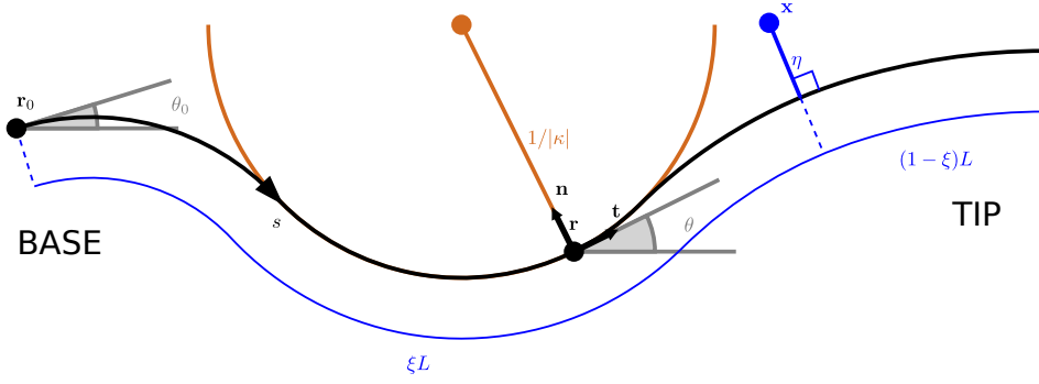
Figure 2: Midline organ representation in two spatial dimensions. The variable s describes distance along the midline (thick black line), which is of total length L . At a point r on the midline of the tissue, t and n are the tangent and normal vectors, respectively. The angle made between the positive x -direction and the tangent is denoted by \theta . The curvature \kappa is the rate of change of \theta with respect to s , or equivalently the reciprocal of the radius of the osculating circle meeting the surface at a point (brown). The variable \xi is the proportion of the distance of a point along the midline in the initial configuration ; a point at constant \xi corresponds to a material point. This coordinate system is extended to points away from the midline through the variable \eta , which is the (signed) distance from a point x to the midline along a line normal to the midline.
