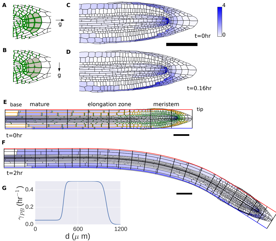
Figure 7: Simulations of gravitropic bending. (a) PIN auxin efflux carriers (green) have apolar localization around the boundary of columella cells (gray) when the root is growing vertically. (b) PINs localize to lower sides of columella cells following change in the relative gravity vector g (i.e. through reorientation of the root). (c) Initial auxin concentrations (blue shading), found from the steady-state of the auxin transport equations (Appendix C) with collumella PINs as in (a). (d) Auxin concentrations at t = 0.16 hr following reorientation of root and change in columella PIN localization. (e) Initial root geometry. Auxin influx and efflux carriers indicated by orange and green lines. Discretized root midline (black) overlaid. (f) Root geometry at t = 2 hr, with bending of the root evident. (g) Step-stool elongation rate function \gamma_{PB} as a function of distance d = L - s from root tip. All scale bars 100 \mu\text{m} . Same colour scale used for auxin concentrations in all panels.
