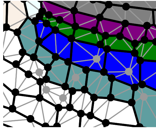
Figure 1: Vertex-based organ representation. Circles indicate vertices. Gray lines show triangulation of the polygonal regions. Gray circles are vertices inserted within cells for the purposes of triangulation. Coloured shading indicates cell type within the organ.
