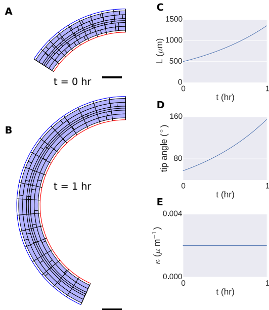
Figure 5: Simulations with curved initial geometry. (a) Initial synthetic curved geometry. (b) Simulation at t = 1 hr. Evolution of length (c), tip angle (d) and average curvature (e). Scale bar 100 \mu\text{m} .
