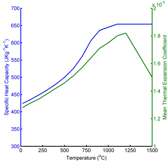
Figure 4: Specific heat and thermal expansion coefficient.
