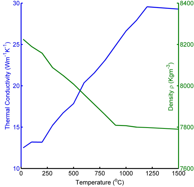
Figure 5: Thermal conductivity and density.
