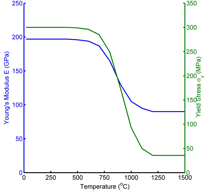
Figure 6: Young's modulus and yield stress.
