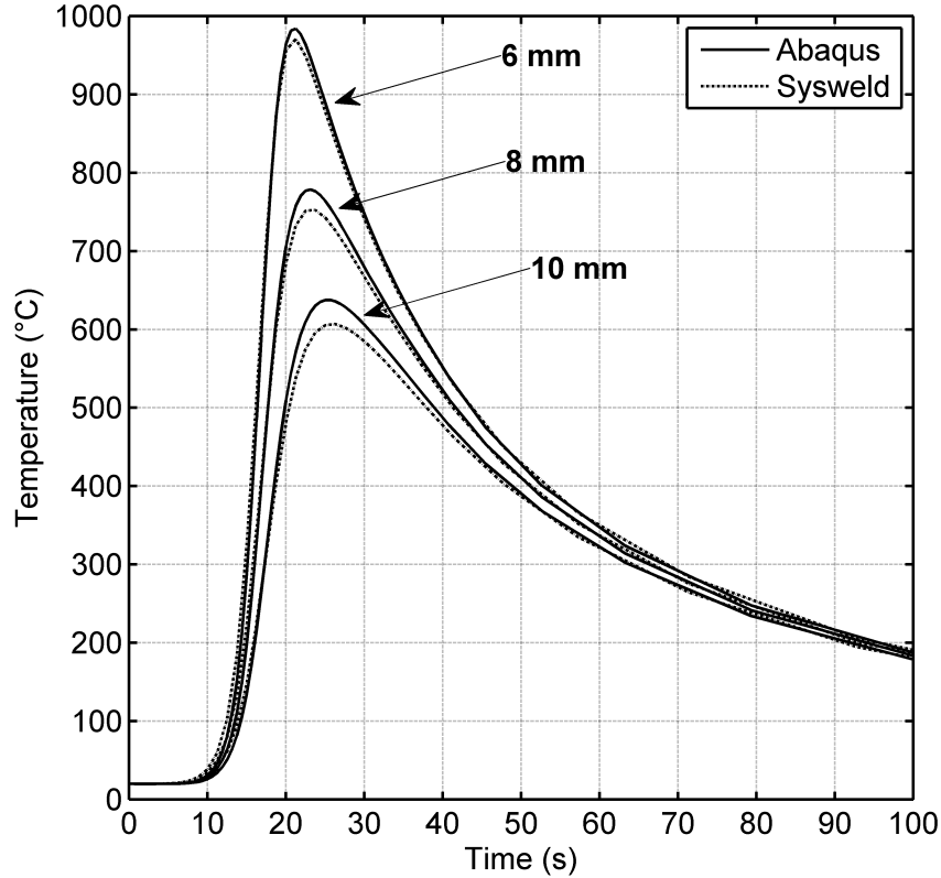
Figure 13: Repairing weld: measured and predicted thermal cycles at 6, 8 and 10 mm from the weld center line at approximately the mid-length of the weld.
