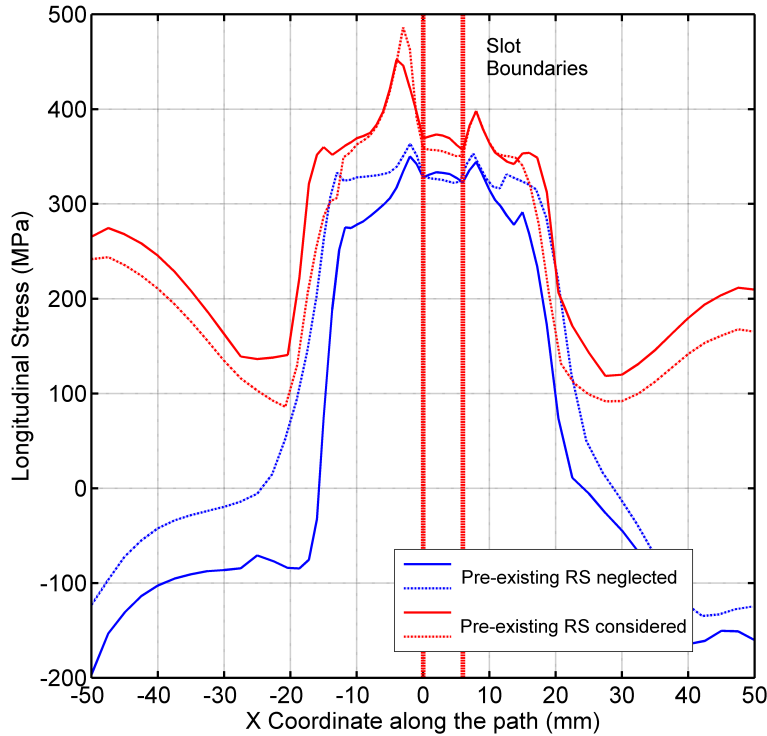
Figure 21: Effect of the initial residual stress on the longitudinal stress. Abaqus (solid line) Sysweld (dashed line).
