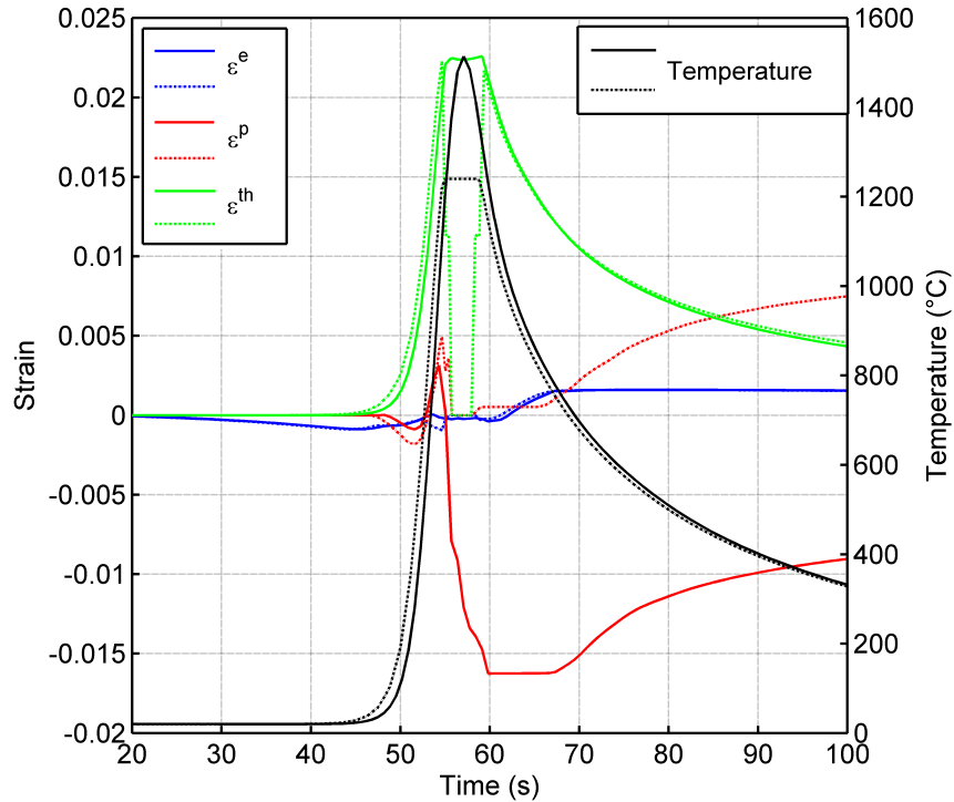
Figure 15: Thermal and strains histories in a point in the weld pool. Abaqus (solid line) Sysweld (dashed line).
