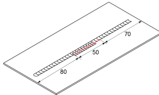
(c) Slot re-filling.
