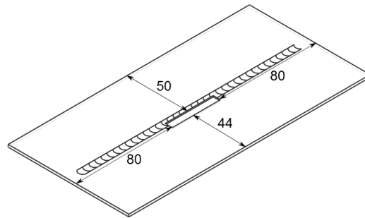
(b) Machining.
