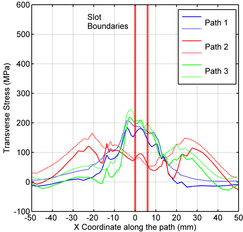
Figure 20: Transverse residual stress after repair procedure. Abaqus (solid line) Sysweld (dashed line).
