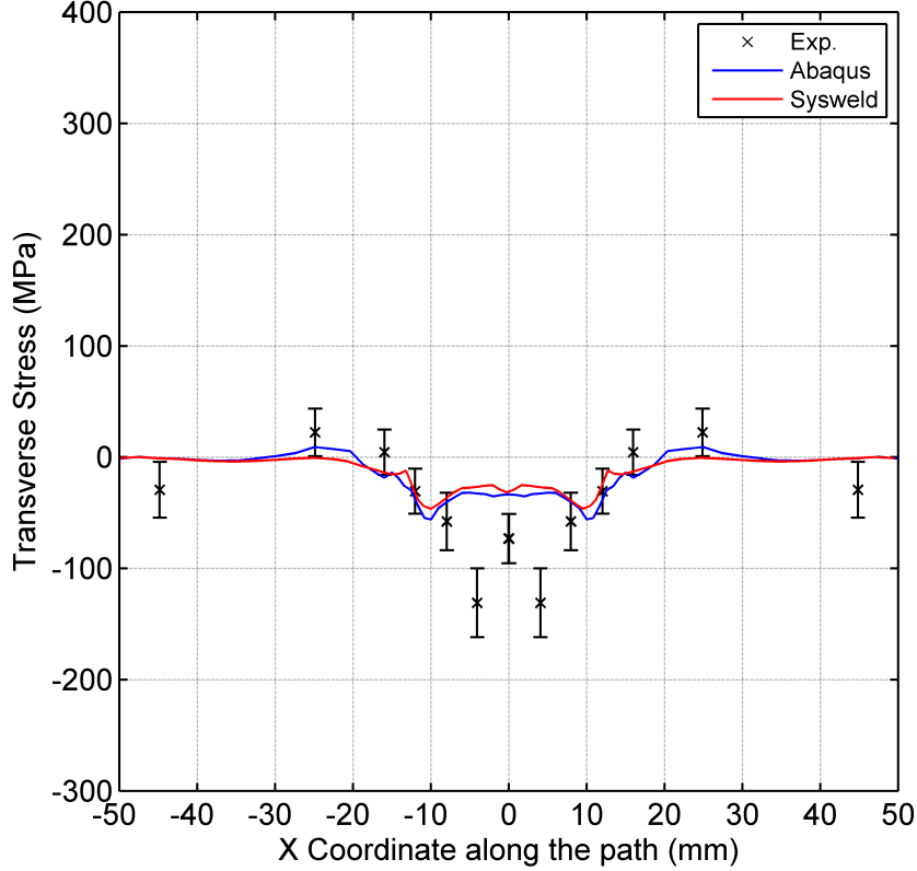
Figure 18: Transverse residual stress after initial weld along path 2'.
