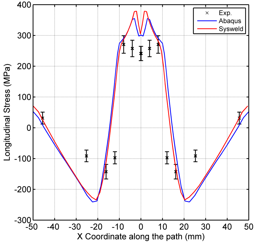
Figure 17: Longitudinal residual stress after initial weld along path 2'.
