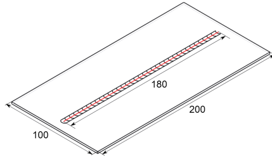
(a) Bead-on-plate weld.
