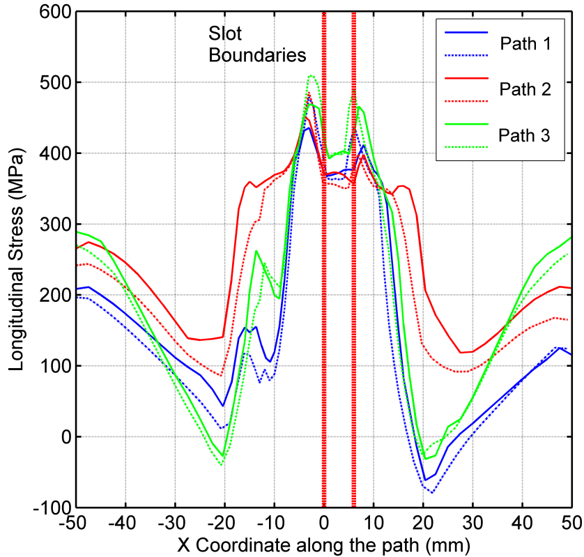
Figure 19: Longitudinal residual stress after repair procedure. Abaqus (solid line) Sysweld (dashed line).
