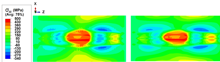
(b) After repair procedure.
