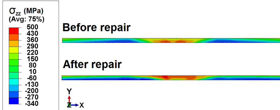
Figure 22: Longitudinal residual stress before and after repair procedure. Cross section at path 2 (Abaqus).
