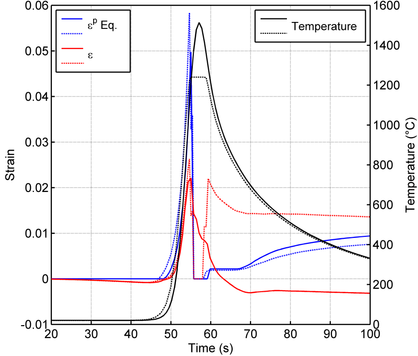
Figure 14: Thermal and strains histories in a point in the weld pool. Abaqus (solid line) Sysweld (dashed line).
