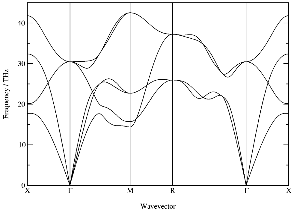
FIG. 6. Dispersion curves for B2 \text{ MgO} at a lattice parameter 2.0 \text{ \AA} . The symmetry points in the dispersion curve are (from left to right) X [\frac{1}{2}00] , \Gamma [000] , M [\frac{1}{2}\frac{1}{2}0] , R [\frac{1}{2}\frac{1}{2}\frac{1}{2}] , \Gamma [000] , and X [\frac{1}{2}00] .
