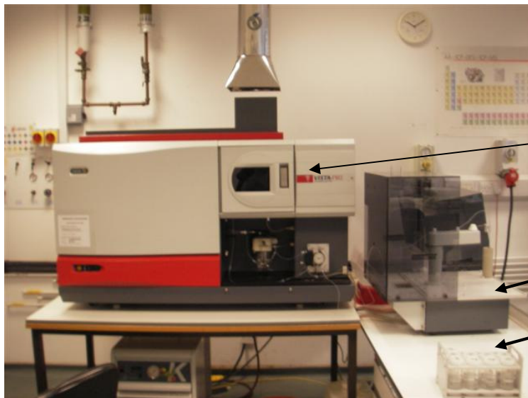
Figure 3.11 The ICP-AES
