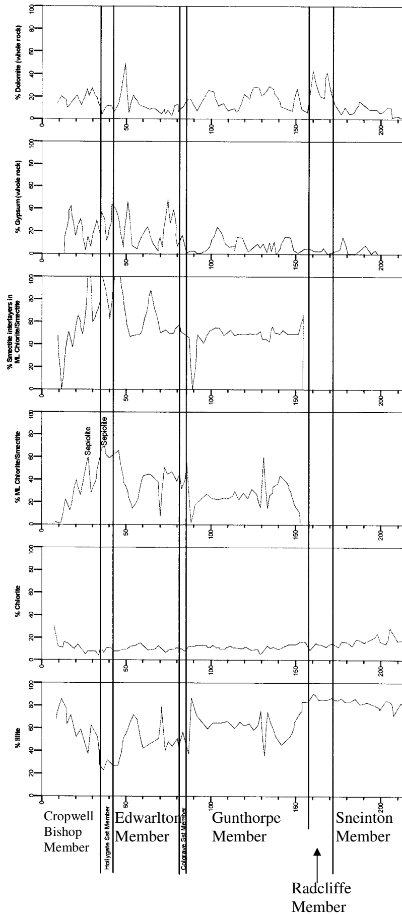
Figure 2.7 The composition of the clay fraction (<2 \mu m) and the whole rock content of gypsum and dolomite of the Mercia Mudstone Group (after Chandler et al. , 2001)
