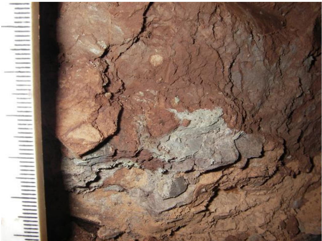
Figure 4.23 Vertical section with green mottling within the remoulded zone around pile MR2, at a depth of 1547mm below ground level
