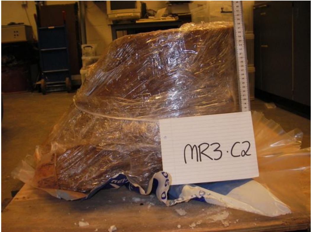
Figure 4.27 The second section from pile MR3 510-860mm below ground level
