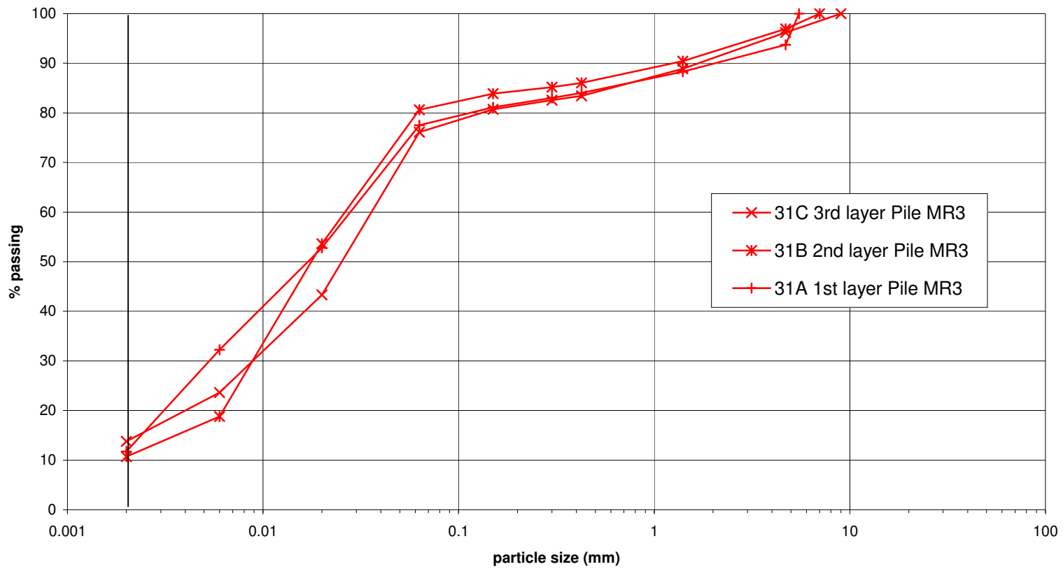
Figure 4.88 PSD curve for samples taken from around pile MR3
