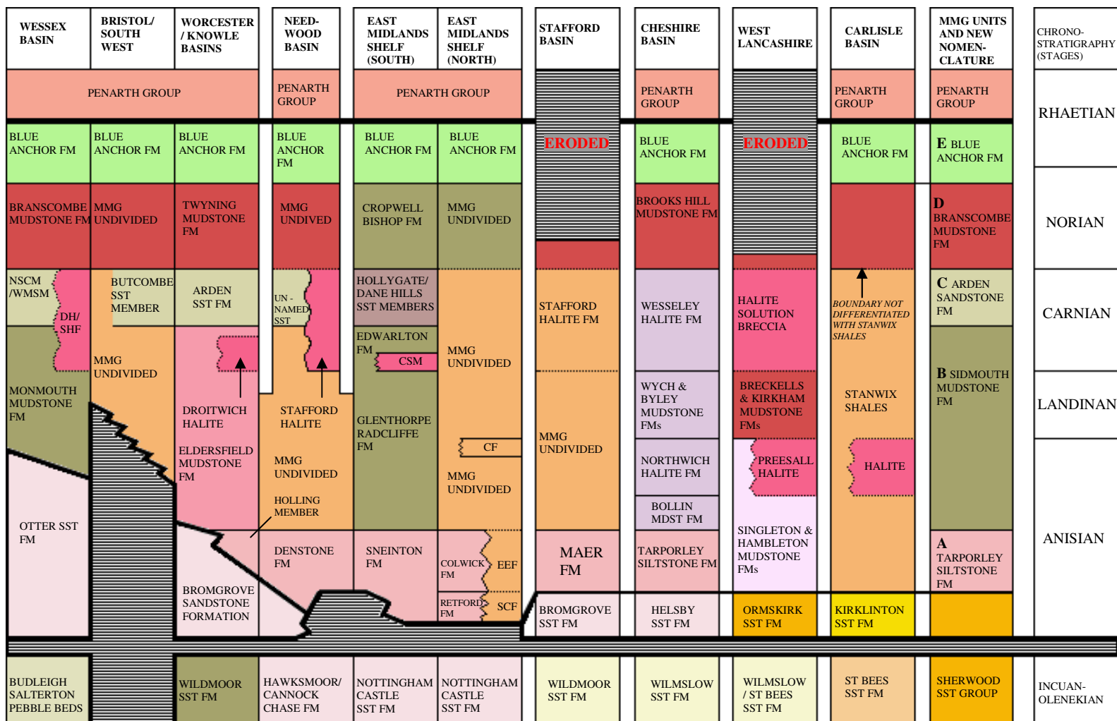
Figure 2.5 UK stratigraphy for the Mercia Mudstone Group comparing the old and new nomenclature (after Howard et al. , 2008). Gaps between columns indicate geographical separation of basins. Broken lines are boundaries seen only in boreholes. CF: Clarborough Formation; CSM: Cotgrave Sandstone Member; DH: Dorset Halite; MMG: Mercia Mudstone Group; NSCM: North Curry Sandstone Member; SCF: Seaton Carew Formation; SHF: Somerset Halite Formation; WMSM: Weston Mouth Sandstone Member; FM: Formation; SST: Sandstone; MDST: Mudstone
