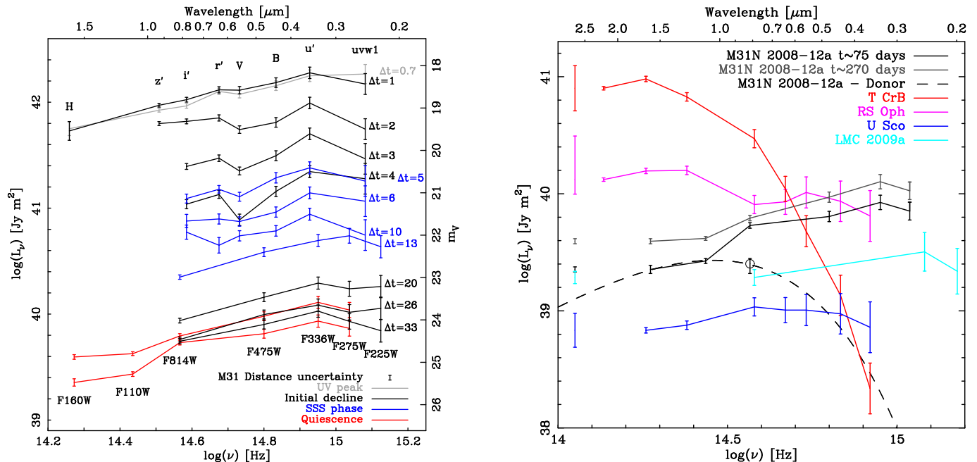
Figure 2. Distance and extinction ( E_{B-V} = 0.1 ; DHG17) corrected SEDs showing Left: the evolving SED of the 2015 eruption (blue points indicate epochs when the SSS emission was visible, red points indicate the archival photometry), and Right: the quiescent M31N 2008-12a compared to the quiescent RNe RS Oph, T CrB, U Sco, and LMC 2009a. The black data shows M31N 2008-12a at minimum ( \sim 75 days post-eruption), and the gray data at an elevated state ( t \simeq 270 d). Throughout, units chosen to allow comparison with similar plots in Schaefer (2010, see their Fig. 71) and DWB14 (see their Fig. 4). The central wavelength locations of the Johnson-Cousins, Sloan, HST , and Swift filters are shown to assist the reader, see the Keys for line identifications. For each system, the photometric uncertainties are relatively small, indicated error bars are dominated by extinction uncertainties, the isolated error bar to the left of each SED indicates the systematic distance uncertainty. The single circled black data point indicates the excess donor flux once the accretion disk model (see Section 4.5) has been subtracted. The dashed black line indicates a power law-fit to the M31N 2008-12a donor SED (see Section 5.2).
