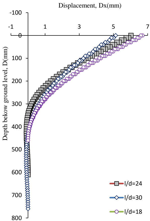
Fig. 4. Piles displacement profile versus depth.
