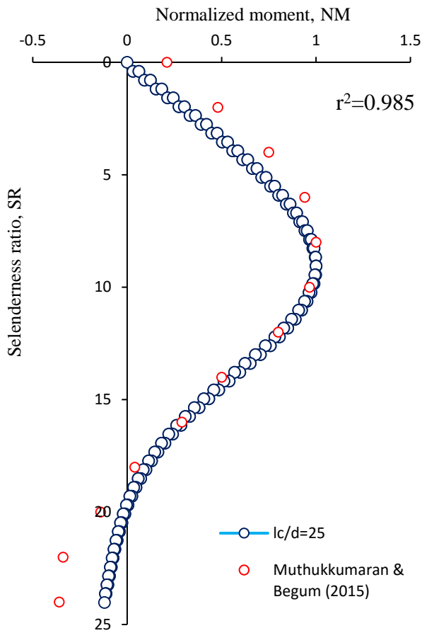
Fig. 6. Piles displacement profile versus depth.
