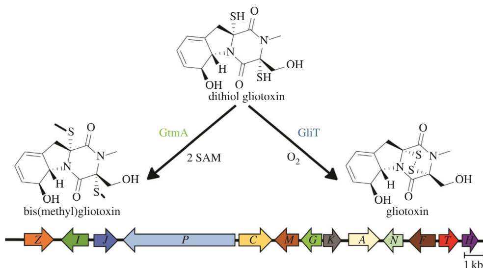
Figure 1. Conversion of gliotoxin between the reduced (dithiol gliotoxin), oxidized (gliotoxin) and bis-thiomethyl forms. In A. fumigatus , the gli -cluster that encodes gliotoxin biosynthesis consists of 13 genes (in colour and labelled with their last letter) and is located on chromosome 6 [4–6]. gtmA is encoded outside the cluster and is on chromosome 2.
