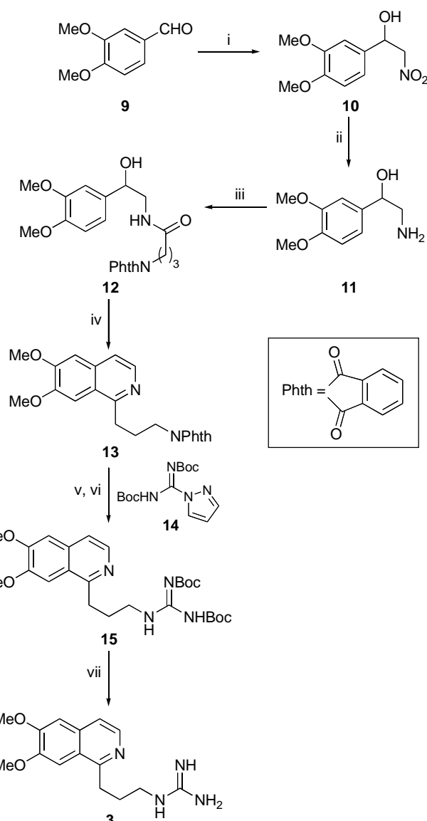
Scheme 3 Reagents and conditions: i. CH 3 NO 2 , 4 Å mol. sieves, DMSO, 85%; ii. H 2 , 10% Pd/C, MeOH, 100%; iii. 4-Phth-aminobutyric acid, EDCI, DMAP, CH 2 Cl 2 , 75%; iv. POCl 3 , Δ, toluene, 66%; v. hydrazine hydrate, Δ, EtOH; vi. 14 , EtN( i -Pr) 2 , MeOH, 82% over two steps; vii. TFA, CH 2 Cl 2 , 73%.
