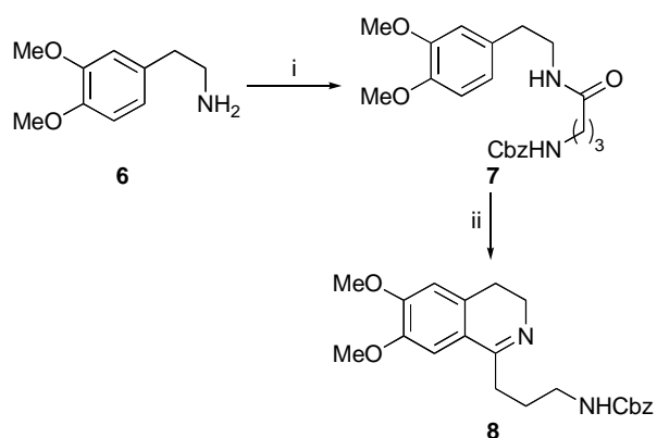
Scheme 2 Reagents and conditions: i. 4-Cbz-aminobutyric acid, EDCI, DMAP, CH 2 Cl 2 , rt, 89%; ii. POCl 3 , Δ, 73%.
