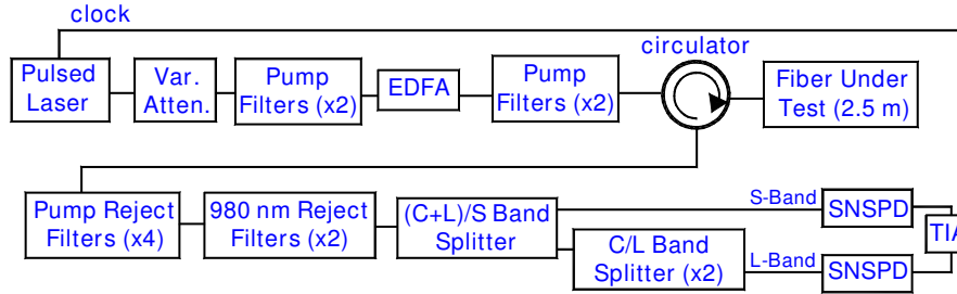
Fig. 1. Diagram of our high-spatial-resolution fiber-optic temperature sensor system. EDFA: erbium-doped fiber amplifier, SNSPD: superconducting nanowire single-photon detector, TIA: time interval analyzer. The pulsed laser is a femtosecond fiber laser with a 36 MHz clock rate. The pump filters are 1 nm linewidth at a wavelength of 1533.47 nm. The pump reject filters are identical to the pump filters, but are connected so that they filter out the pump wavelength. The (C + L)/S bandsplitter separates the S-band wavelengths (1460 nm –1490 nm) from the C-band wavelengths (1530 nm –1565 nm) and L-band wavelengths (1570 nm –1610 nm). The C/L bandsplitter separates the L-band wavelengths from the C-band wavelengths.
