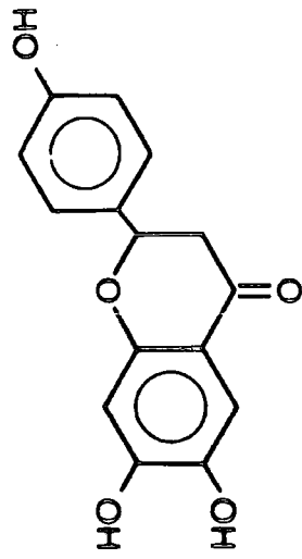
Apigenin
