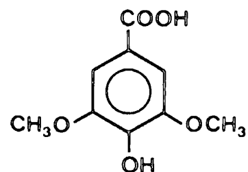
Syringic acid
