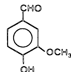
Vanillin
