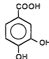
3,4 dihydroxy - benzoic acid
