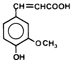
Ferulic acid
