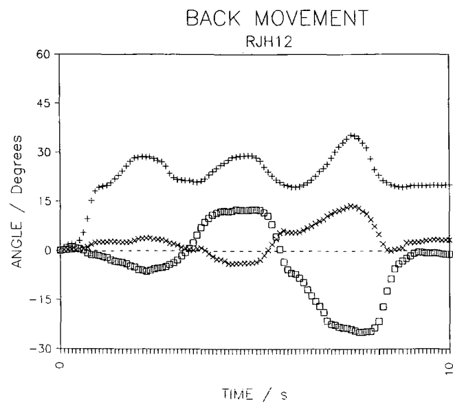
Figure 5 The movements of a subject performing axial rotation whilst sitting; +, flexion; □, bend +ve L; ×, twist +ve L
