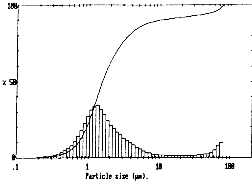
Fig. 35 Particle size distribution of AJ-1/23 C-2 after stirring for 75 min. to break up flocs
