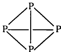
Figure 1.4: White phosphorus.
