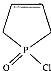
Figure 2.5: 1-Chloro-1-oxo-3-phospholene.
