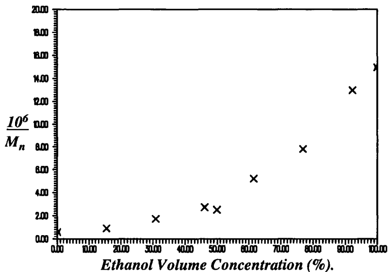
Figure 3.9: Graph of reciprocal number average molecular weight against ethanol volume concentration (%) for the ROMP of dimethyl bicyclo[2.2.1]hept-2-ene-5-phosphonate using \text{RuCl}_3 \cdot 3\text{H}_2\text{O} and ethanol/water.
