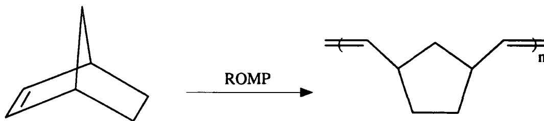
Figure 1.12: Ring Opening Metathesis Polymerisation of norbornene.
