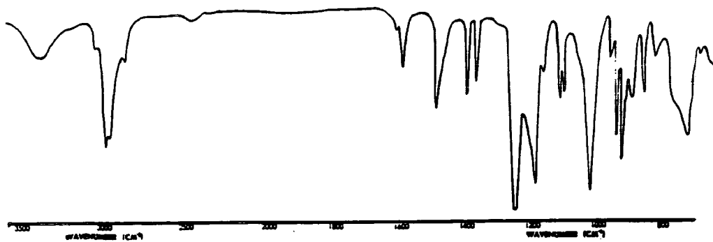
Appendix D5: 1-Neopentoxy-1-oxo-3-phospholene.
