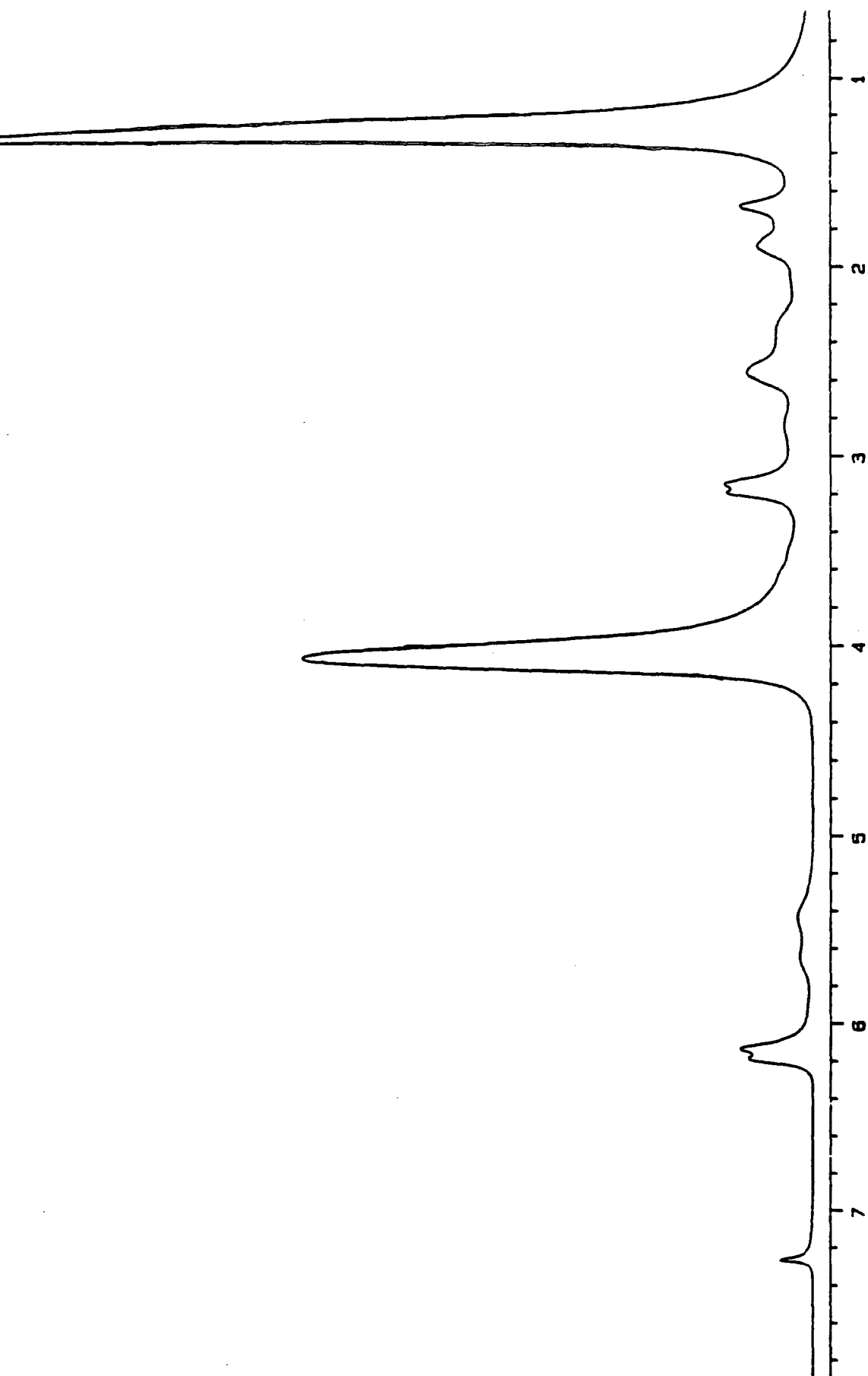
Appendix A15: ^1\text{H} NMR Spectrum (399.952 MHz) of Poly[2,5-[3,4-bis(diethylphosphonate)]-cyclopentylene]-vinylene.
