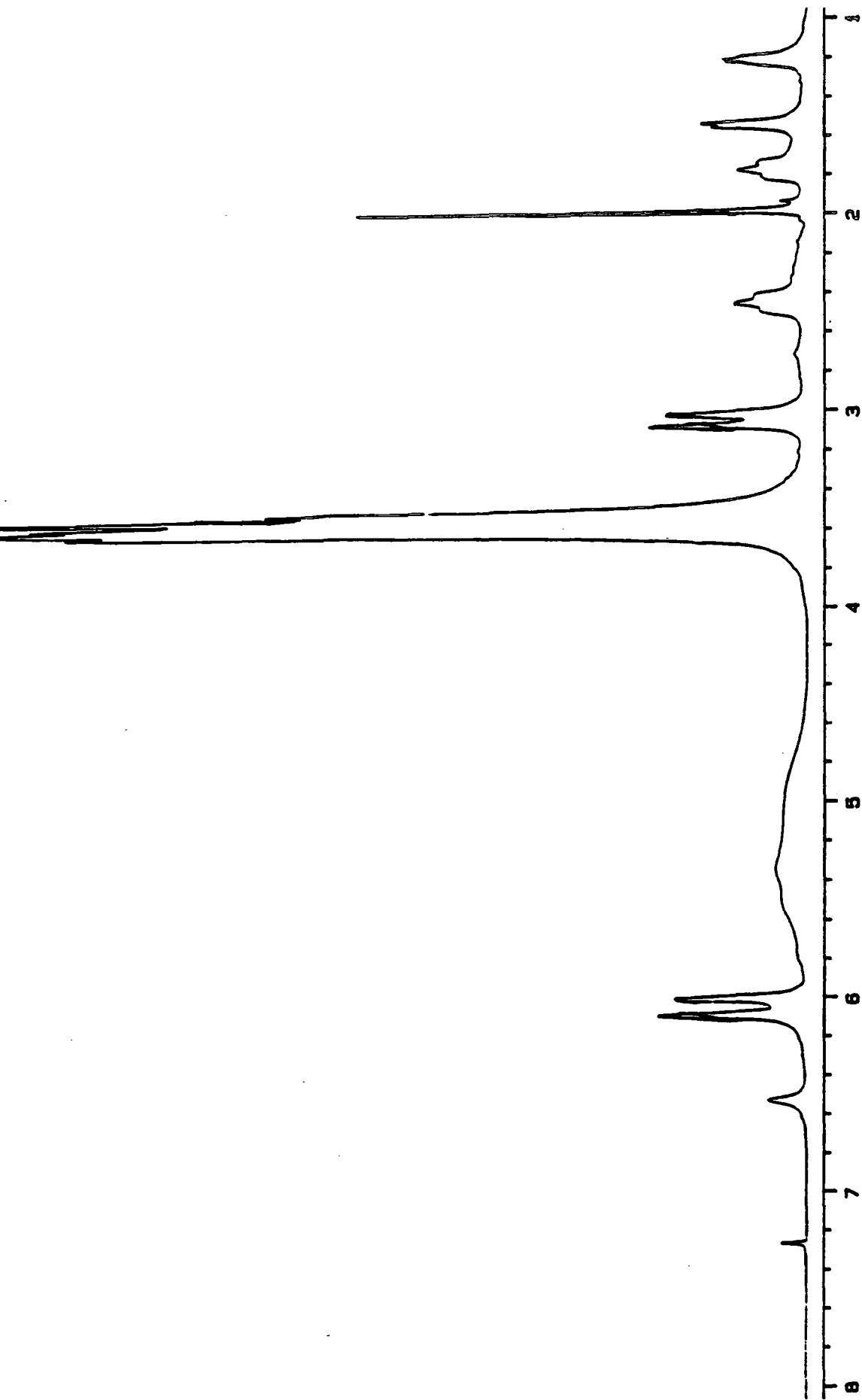
Appendix A14: ^1\text{H} NMR Spectrum (399.952 MHz) of Poly[2,5-[3,4-bis(dimethylphosphonate)]-cyclopentylene]-vinylene.
