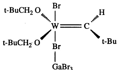
Figure 1.20: The Osborn catalyst.
