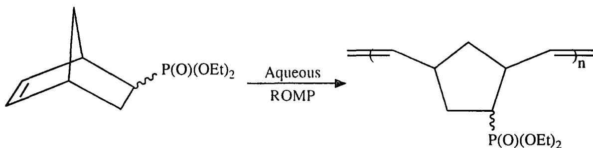
Figure 3.12: Aqueous ROMP of diethyl bicyclo[2.2.1]hept-2-ene-5-phosphonate.
