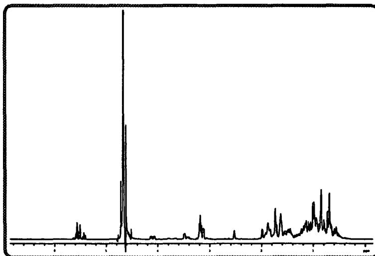
Figure 2.18: 1 H spectrum of hydrolysis product (399.952 MHz/D 2 O).
