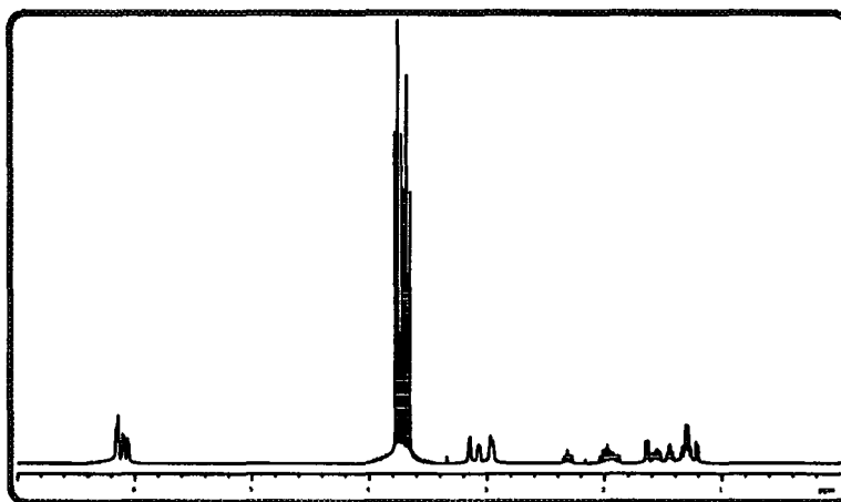
Figure 2.17: 1 H spectrum of dimethylbicyclo[2.2.1]hept-2-ene-5-phosphonate (399.952 MHz/CDCl 3 ).
