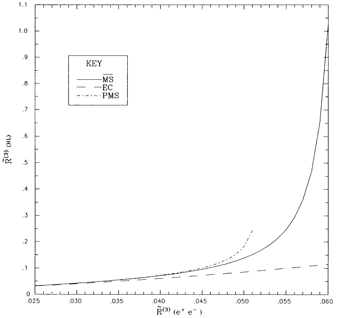
Figure 6.10 \tilde{R}_{\text{HL}} vs \tilde{R}_{e^+e^-} at third order for three RS's.
