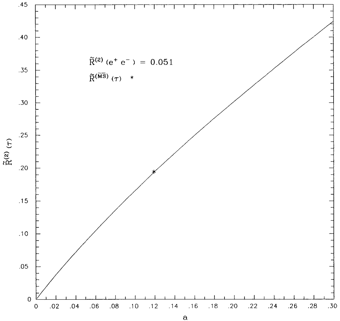
Figure 6.7 \tilde{R}_\tau^{(2)} as a function of the couplant, a , at \tilde{R}_{e^+e^-} = 0.051 , the central value of the Marshall fit. \tilde{R}_\tau^{(2)}(\overline{\text{MS}}) is indicated by an asterisk.
