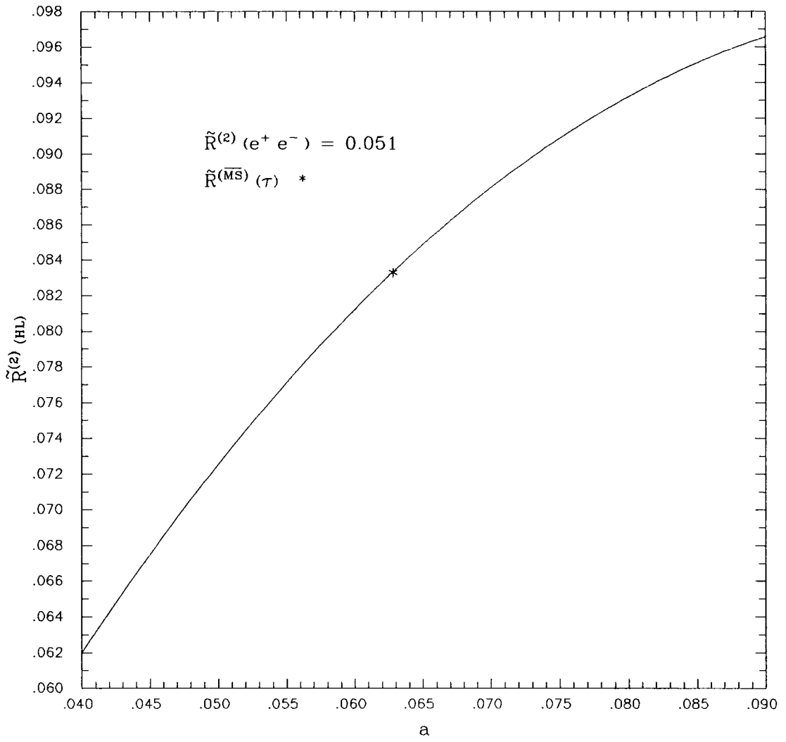
Figure 6.11 \tilde{R}_{HL}^{(2)} as a function of the couplant, a , at \tilde{R}_{e^+e^-} = 0.051 , the central value of the Marshall fit. \tilde{R}_{HL}^{(2)\overline{MS}} is indicated by an asterisk.
