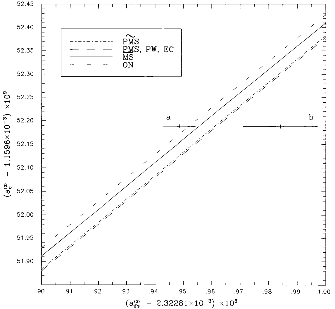
Figure 7.2 The third order approximants to the anomalous magnetic moment of the electron, a_e^{(3)} , for six RS's are plotted as a function of the fine structure constant, a_{fs} . Data point a is that measured from the quantum Hall effect, while data point b is measured from the Josephson frequency and the proton gyromagnetic ratio. As at second order, the optimized approximants, to this accuracy, are identical, with the exception of \widetilde{\text{PMS}} .
