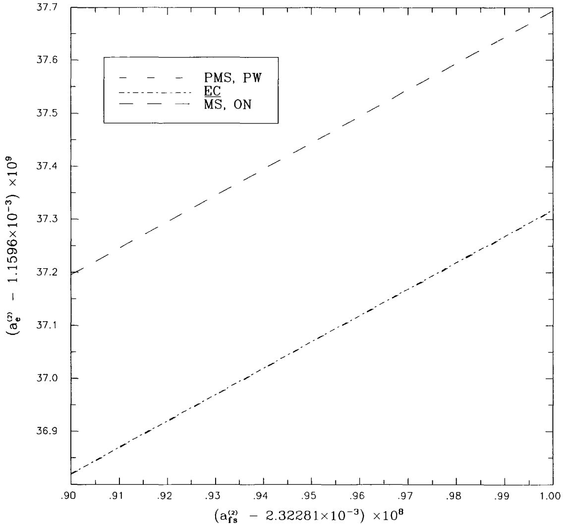
Figure 7.1 The second order approximants to the anomalous magnetic moment of the electron, a_e^{(2)} , for five RS's are plotted as a function of the fine structure constant, a_{fs} . Note that the \overline{MS} and ON approximants are identical as they should be at this order.
