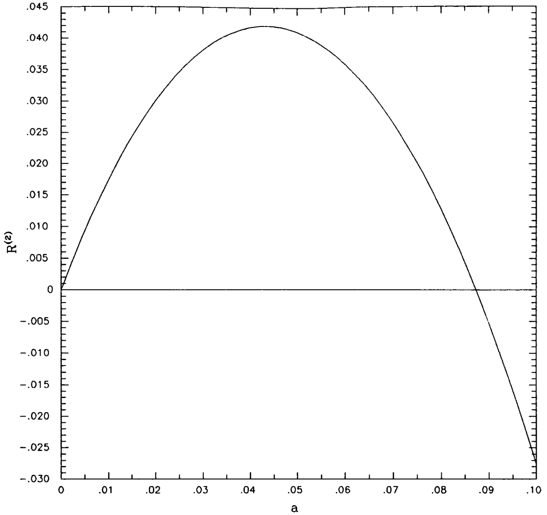
Figure 4.1 R^{(2)} as a function of the couplant, a . This is the general shape that R^{(2)} will have, regardless of the physical process, provided \rho_0 > 0 .
