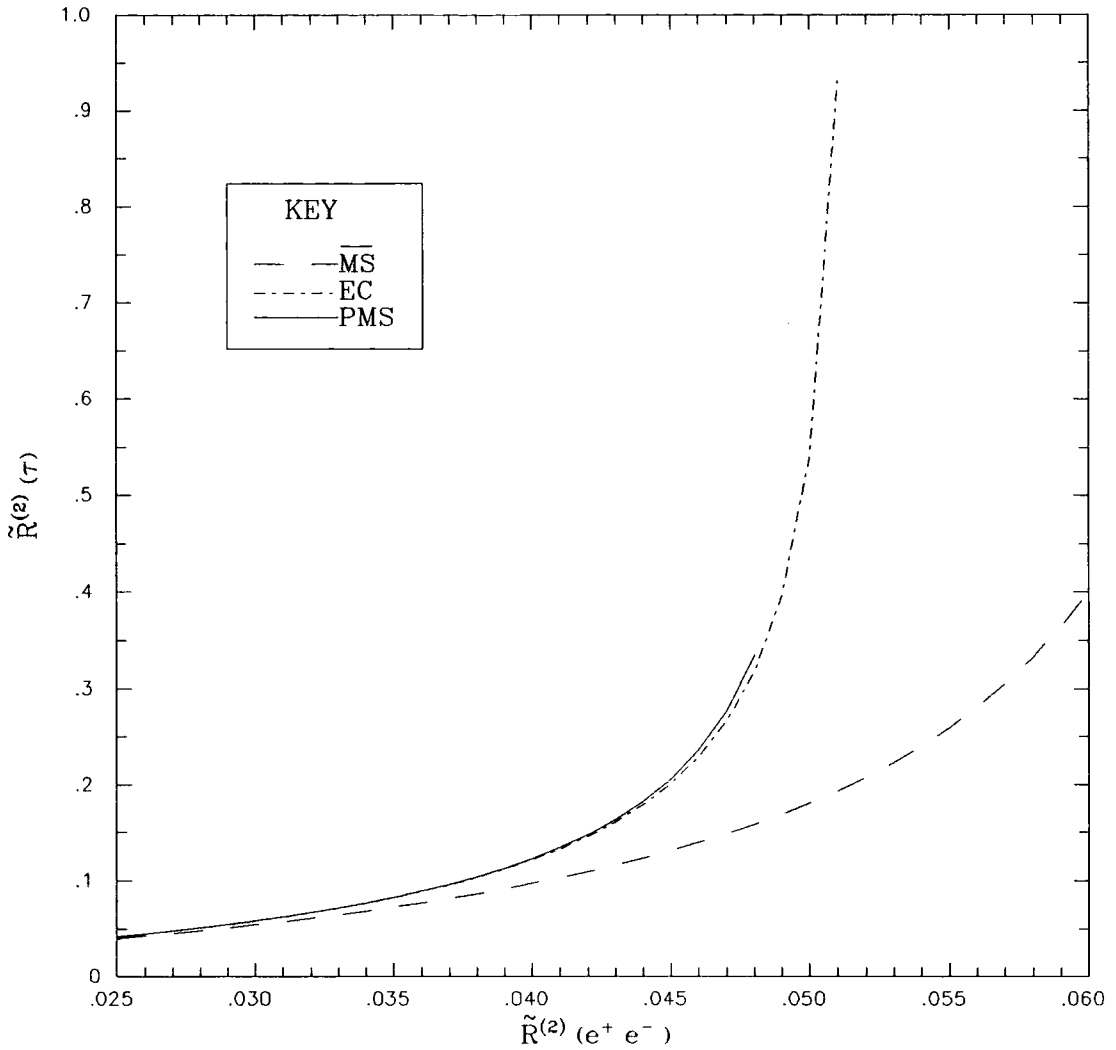
Figure 6.5 \tilde{R}_\tau vs \tilde{R}_{e^+e^-} at second order for three RS's.
