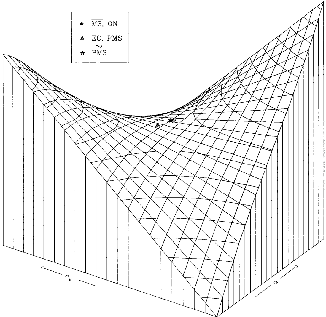
Figure 7.3 a_e^{(3)} as a function of the couplant, a , and the second \beta -function coefficient, c_2 , with 2.3 \times 10^{-3} \leq a \leq 2.34 \times 10^{-3} and -50 \leq c_2 \leq 50 . The values predicted by PMS, EC, \overline{\text{MS}} , ON and \widetilde{\text{PMS}} are indicated. The minimum value of a_e^{(3)} is 1.159\,645\,97 \times 10^{-3} and the maximum value is 1.159\,657\,96 \times 10^{-3} .
