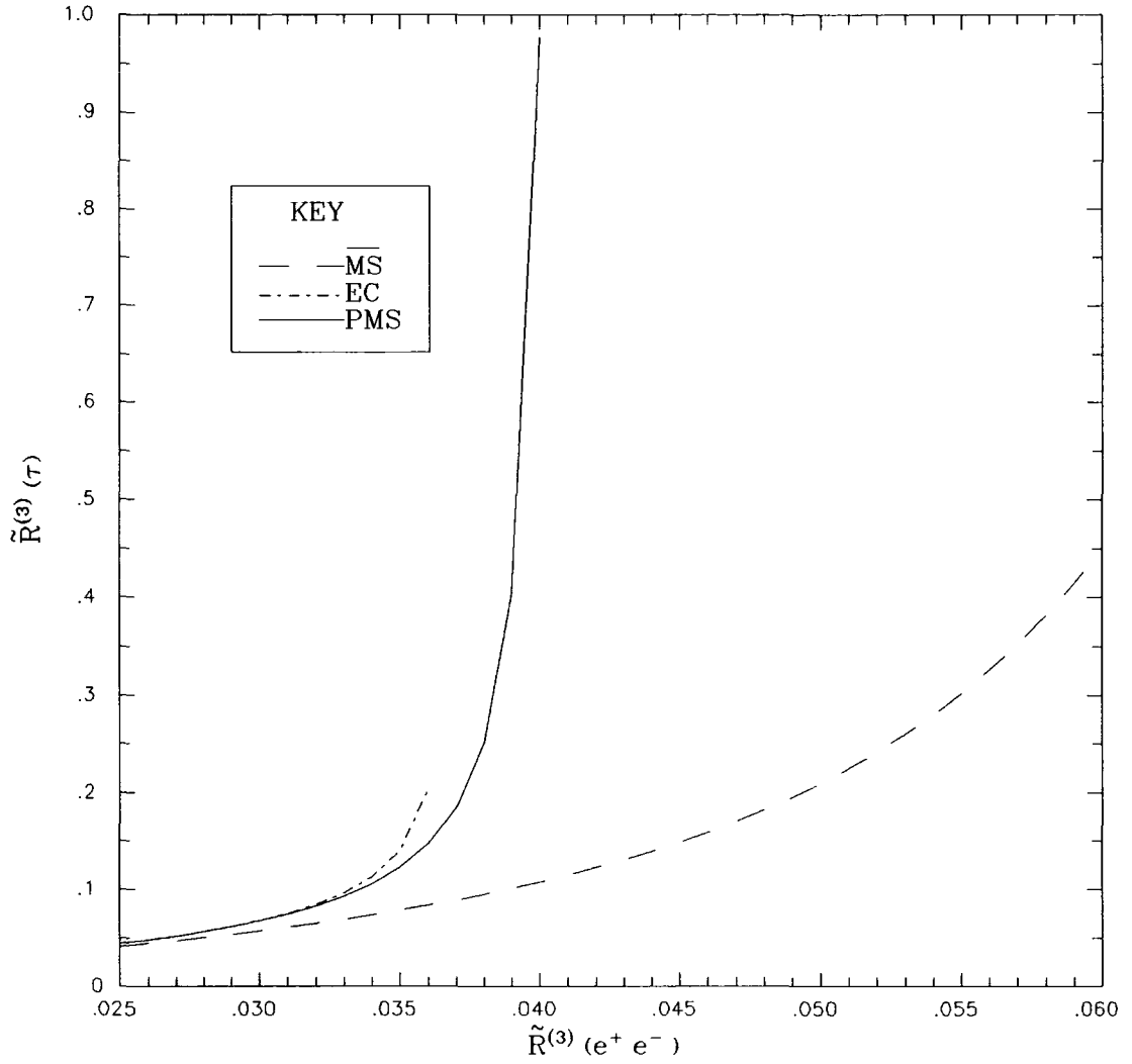
Figure 6.6 \tilde{R}_\tau vs \tilde{R}_{e^+e^-} at third order for three RS's.
