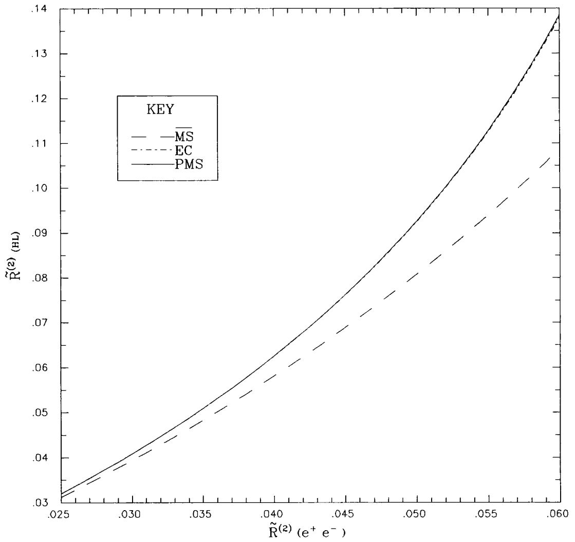
Figure 6.9 \tilde{R}_{HL} vs \tilde{R}_{e^+e^-} at second order for three RS's.
