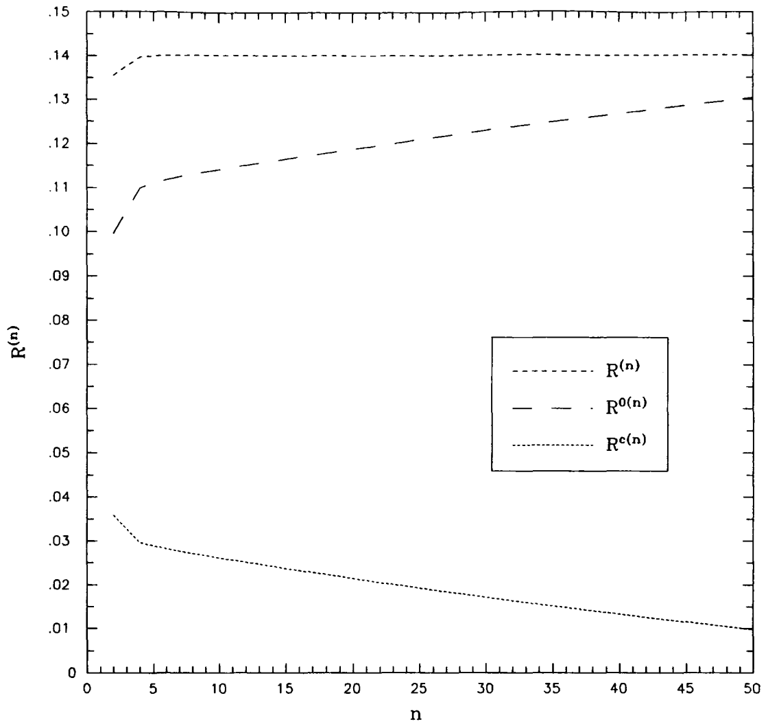
Figure 4.8 R^{(n)}(\widetilde{\text{PMS}}) , R^{0(n)}(\widetilde{\text{PMS}}) and R^{c(n)}(\widetilde{\text{PMS}}) are shown for n = 2, \dots, 50 for the alternating factorial example, with \tau_0 = 4 and for c = 1.26 , showing that R^{0(n)}(\widetilde{\text{PMS}}) tends to R^{(n)}(\widetilde{\text{PMS}}) as n \rightarrow \infty , and R^{c(n)}(\widetilde{\text{PMS}}) tends to 0.
