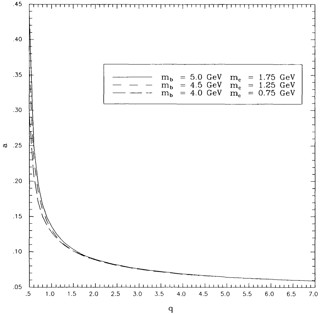
Figure 6.4 The couplant, a , as a function of momentum, q , for three combinations of the mass of the charm and bottom quarks, with \tilde{\Lambda}_{\overline{\text{MS}}}^{(5)} = 0.2 \text{ GeV} , as this \tilde{\Lambda}_{\overline{\text{MS}}} yields the central value of the Marshall fit for \tilde{R}_{e^+e^-}^{(3)} at s = 1000 \text{ GeV}^2 .
