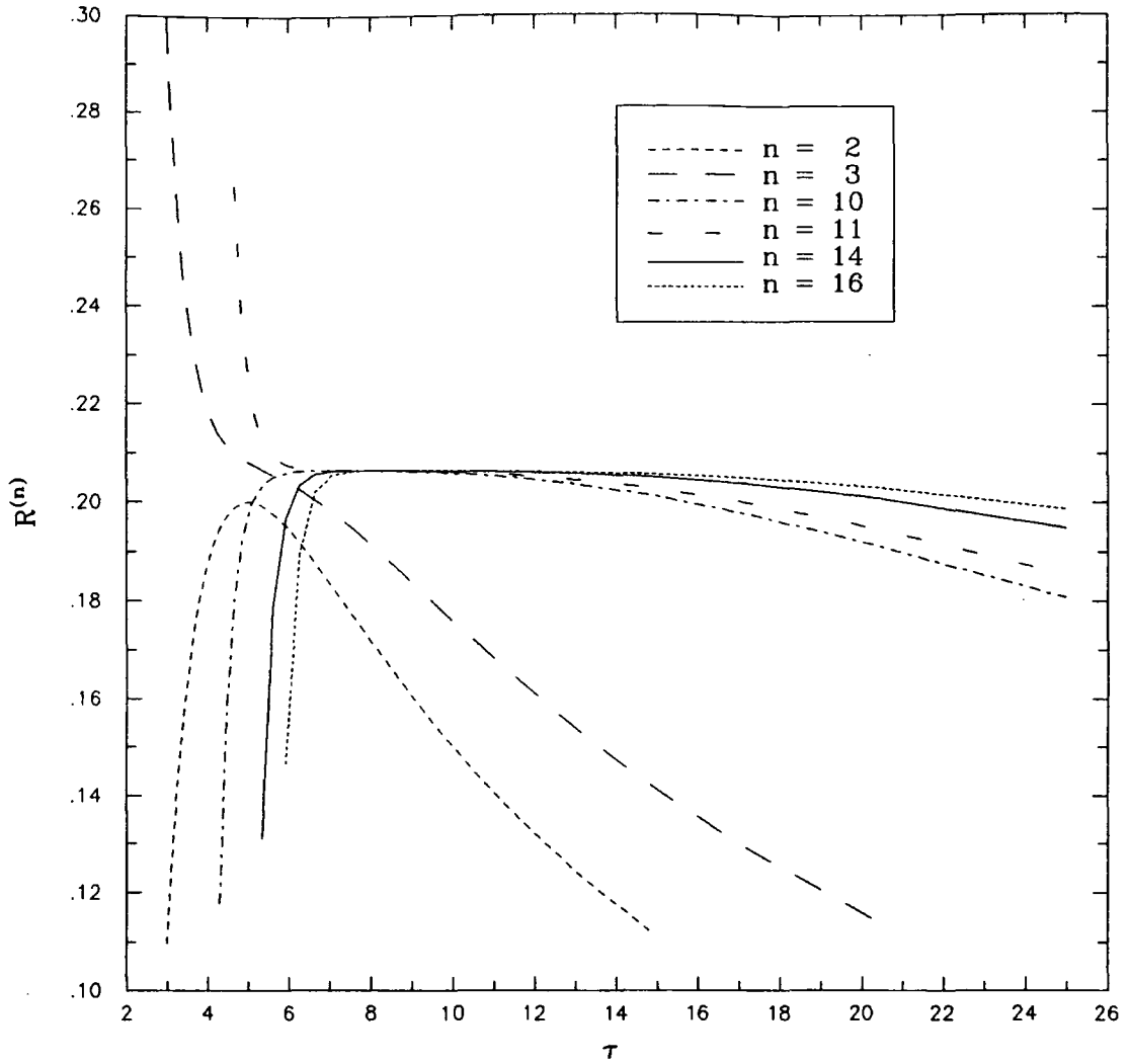
Figure 4.3 R^{(n)} vs \tau for six values of n , showing the plateau region around \bar{\tau}_n moving off to large \tau , and growing in the process.
