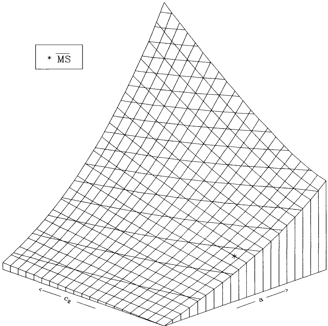
Figure 6.8 \tilde{R}_r^{(3)} as a function of the couplant, a , and the second \beta -function coefficient, c_2 , with 0.044 \leq a \leq 0.144 and -10 \leq c_2 \leq 190 , at \tilde{R}_{e+e-} = 0.051 . \tilde{R}_r^{(3)}(\overline{\text{MS}}) is indicated by an asterisk. The minimum value of \tilde{R}_r^{(3)} for this graph is 0.103, and the maximum is 0.868.
