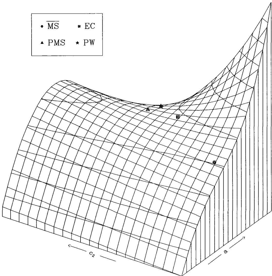
Figure 6.2 \tilde{R}_{e^+e^-}^{(3)} as a function of the couplant, a , and the second \beta -function coefficient, c_2 with 0.02 \leq a \leq 0.07 and -10 \leq c_2 \leq 190 . The values predicted by PMS, EC, PW, and \overline{\text{MS}} are marked. Note that there is no stationary point of inflexion along the c_2 = 0 line, corresponding to no solution to the PMS condition. The minimum value of \tilde{R}_{e^+e^-}^{(3)} for this graph is 3.75 \times 10^{-2} , and the maximum is 7.09 \times 10^{-2} .
