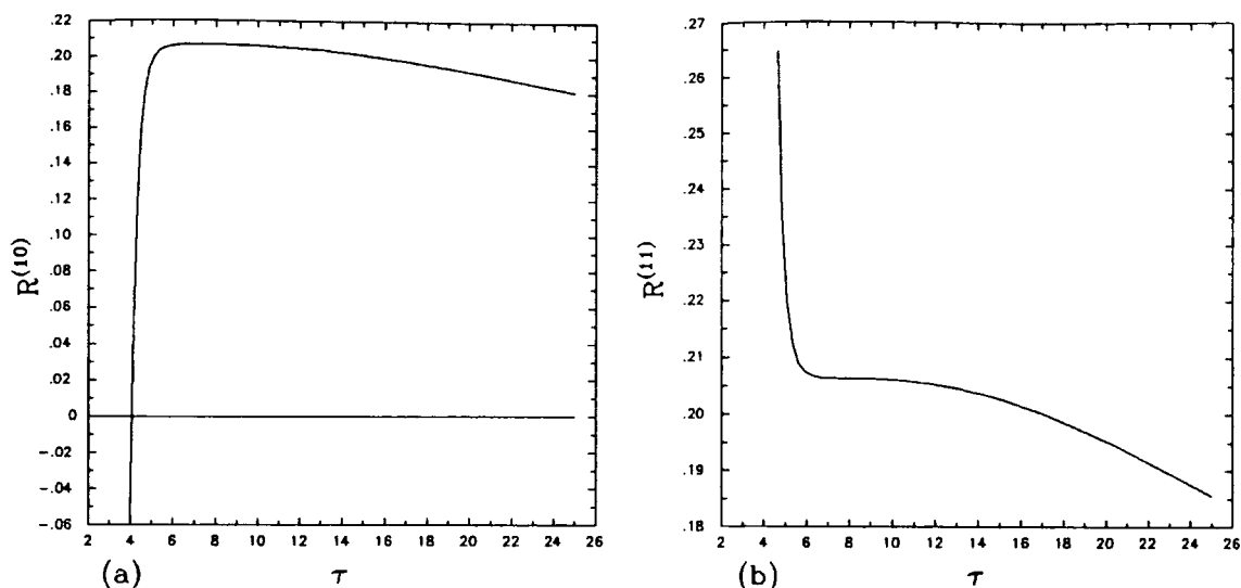
Figure 4.2 R^{(n)} , for n even, will have the shape shown in figure (a), while for n odd, R^{(n)} will have the shape given in figure (b).
