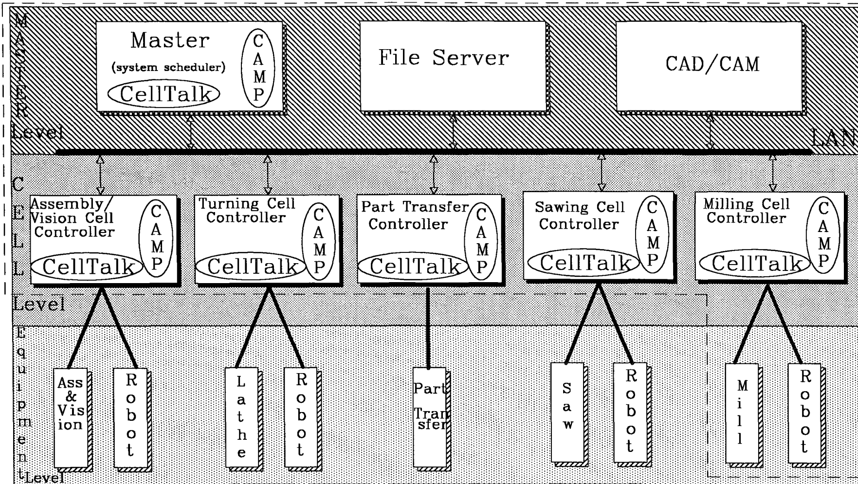
Figure (2-8) Control organisation in Durham FMS. Broken line indicates boundary of the hardware implementation; activities in other cells were emulated for demonstration.
