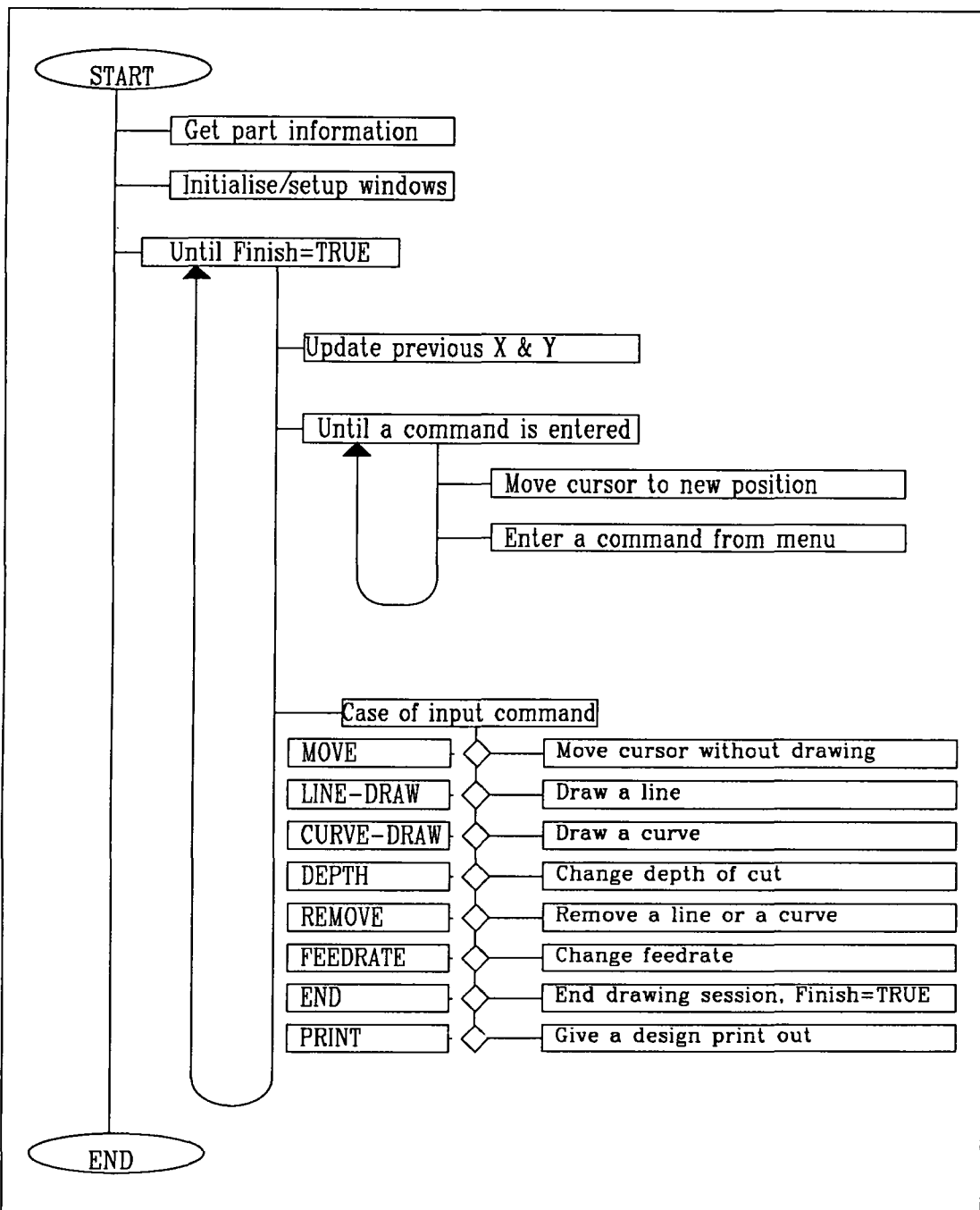
Figure (B-2) A flowchart for design for manufacture module.
