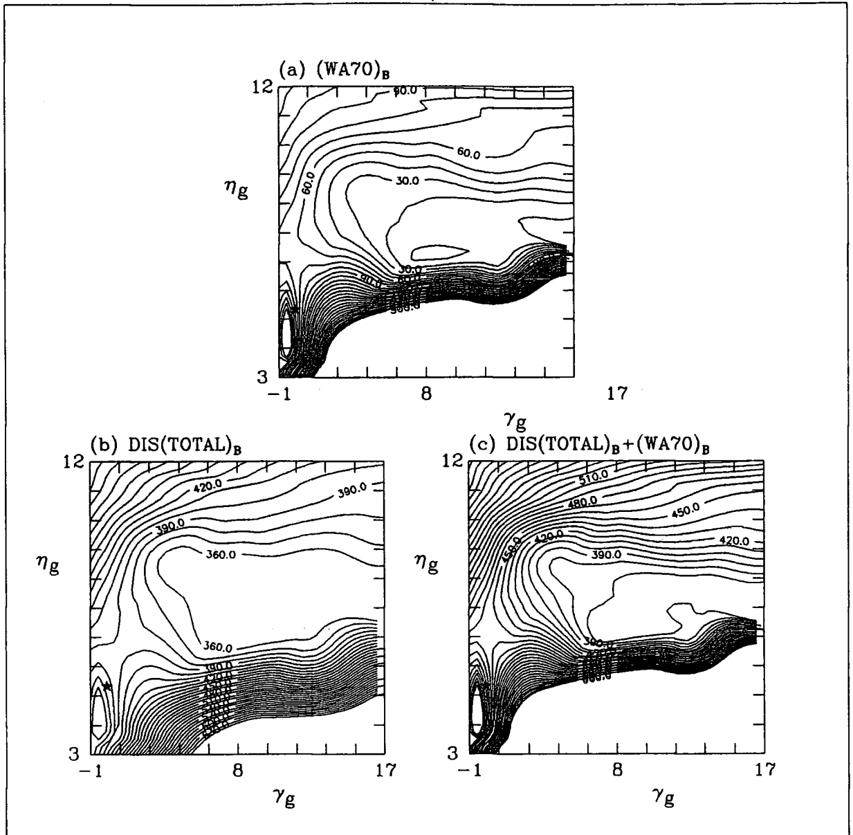
Figure 9.5 (a) shows contours of constant \chi^2 in the \gamma_g - \eta_g plane where \chi^2 is a measure of the quality of the theoretical prediction for the WA70 prompt photon data [66] in the range -0.35 < x < 0.45 (corrected to y = 0 ) using the various sets of parton distributions obtained by re-evolving the HMRS(B) set with the gluon momentum redistributed in the form xg(x, Q_0^2) = A_g x^{\delta_g} (1-x)^{\eta_g} (1 + \gamma_g x) with \delta_g fixed at zero. (b) shows the total \chi^2 to the deep-inelastic scattering data of [32] (BCDMS F_2^{\mu p} ), [36] ( F_2^{\nu N} and x F_3^{\nu N} ) and [40], [42], [43] ( F_2^{\mu n} / F_2^{\mu p} ). (c) is the total of (a) and (b). The stars signify the position of the HMRS(B) fit. The statistical and systematic errors of all data have been combined in quadrature. The contour interval is 10 units of \chi^2 for all three contour plots.
