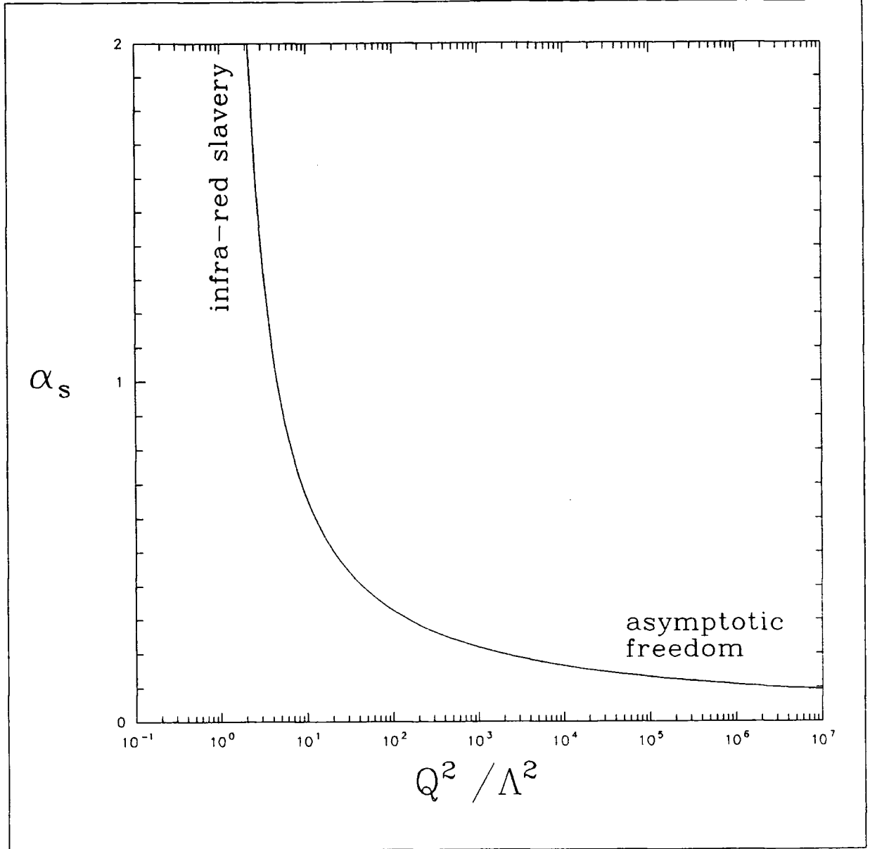
Figure 3.7 The running coupling constant of QCD in the leading logarithm approximation showing the two extreme behaviours at low and high Q^2/\Lambda^2 .
