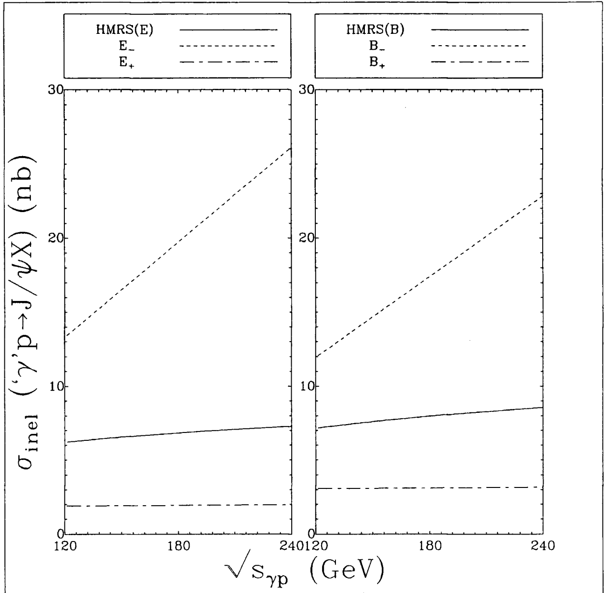
Figure 9.11 The left-hand column shows the predictions for the inelastic J/\psi production cross section, using the three gluons: E (continuous line), E_+ (dot-dashed line) and E_- (dashed line), as a function of \sqrt{s_{\gamma p}} relevant to HERA energies and the right-hand column shows the same for the corresponding B (continuous line), B_+ (dot-dashed line) and B_- (dashed line) gluons. An energy cut of E_\psi < 0.8E_\gamma and a momentum cut of p_T^2 > 0.1m_\psi^2 have been applied.
