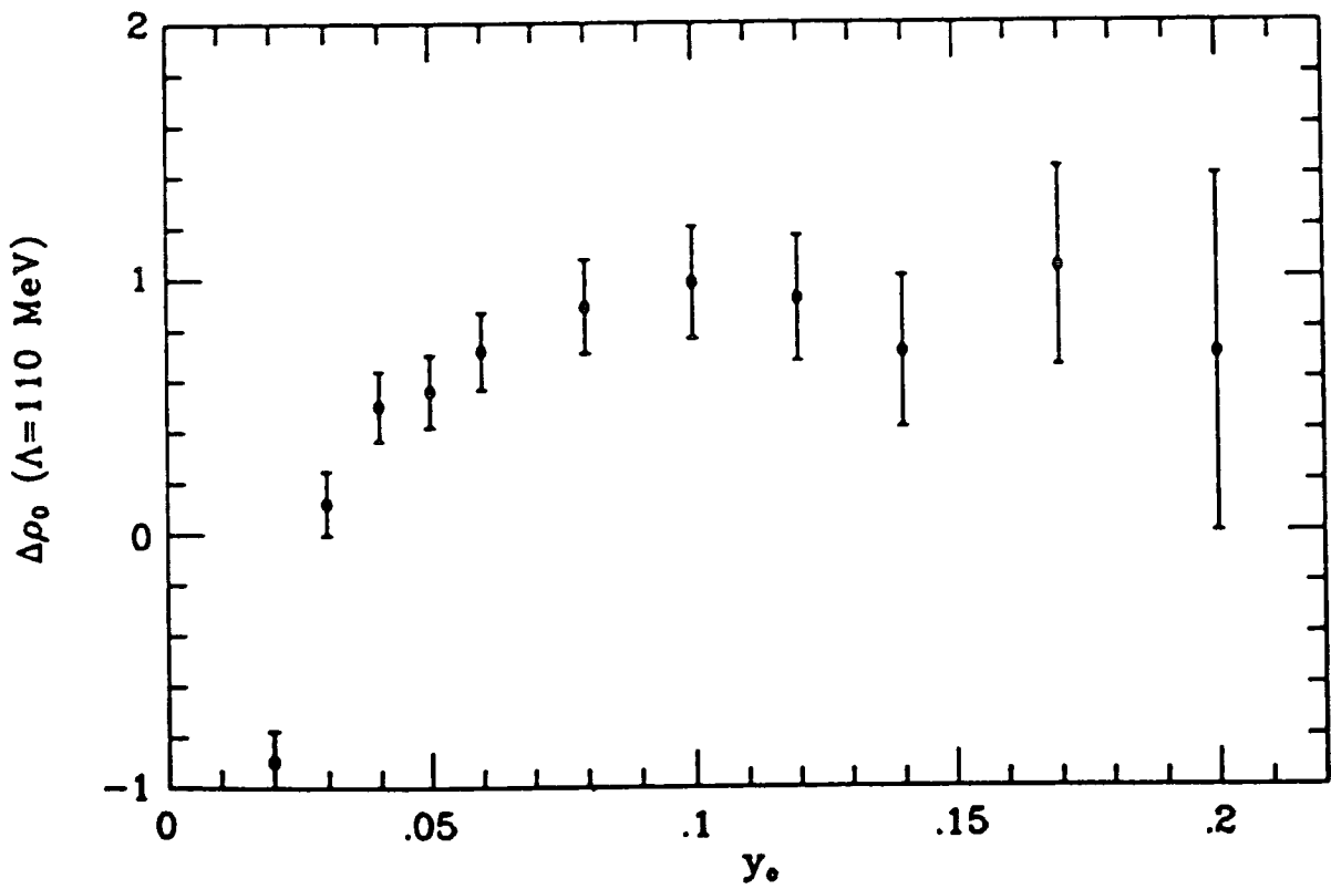
Figure 3.3 \Delta\rho_0 for E0 3-jet fraction
