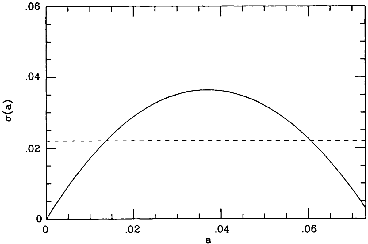
Figure 3.1 Scale Dependence of \sigma^{(2)}
