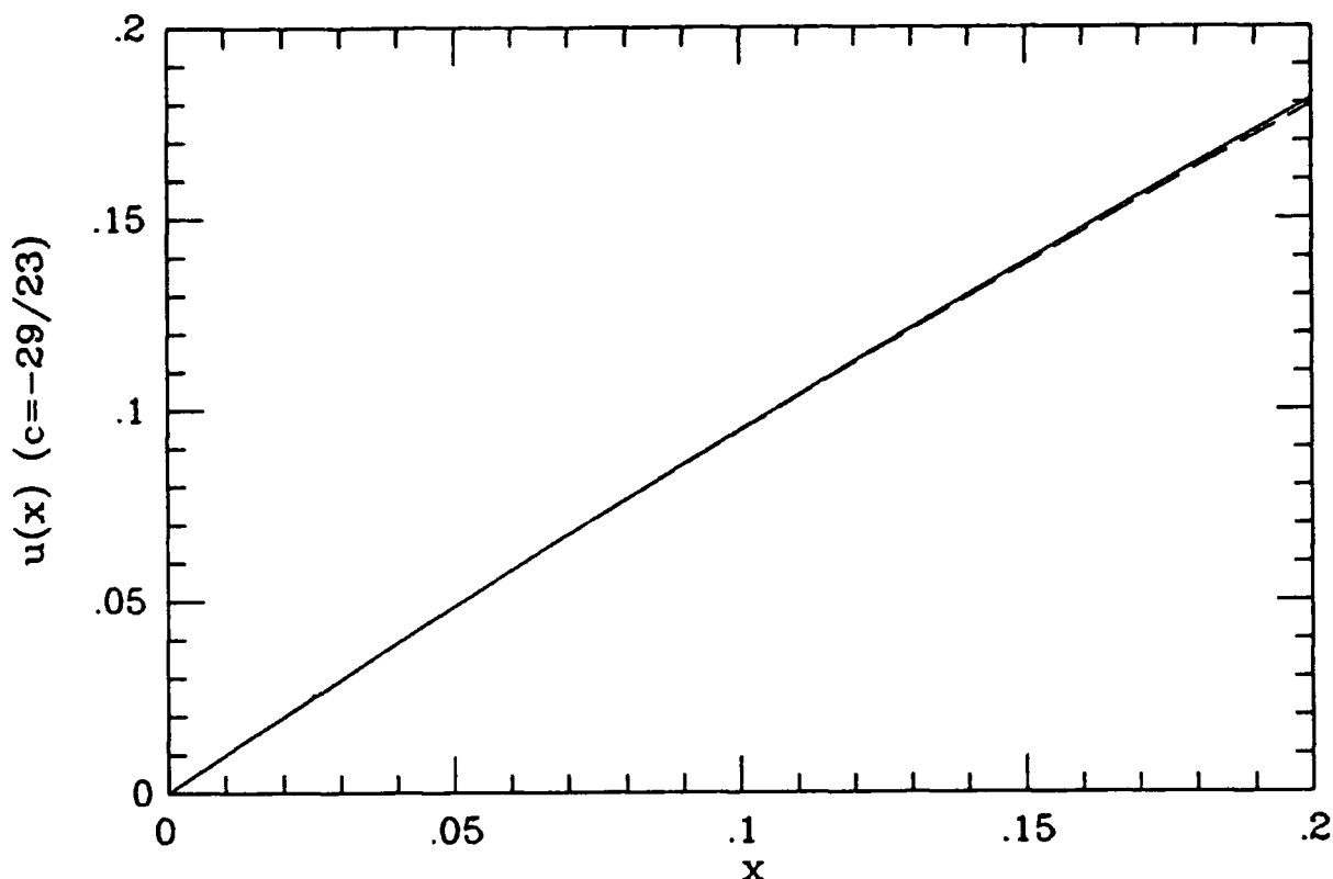
Figure 7.4 Numerical results for c < 0 together with bound.
