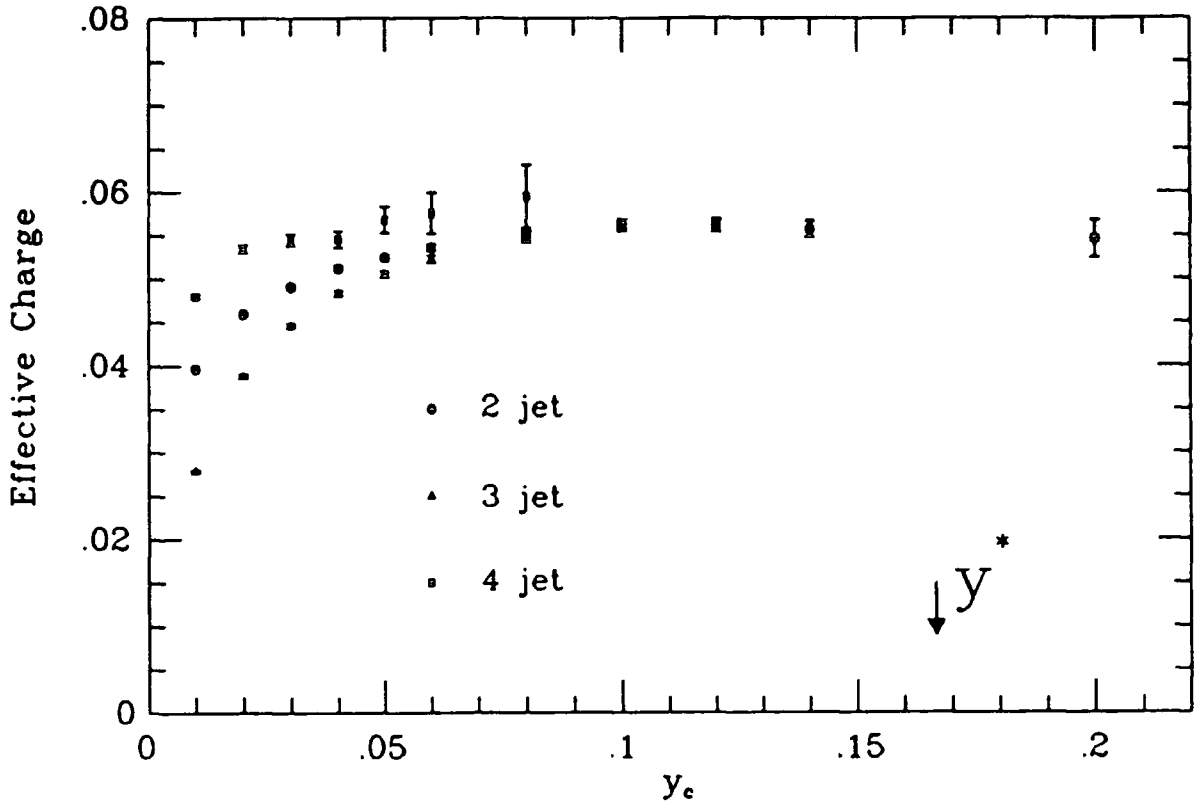
Figure 5.1 E0 effective charges
