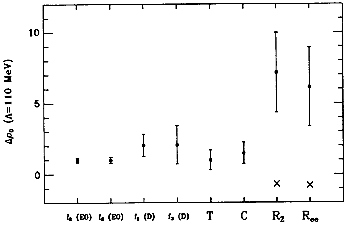
Figure 3.2 \Delta\rho_0 for selected observables assuming \bar{\Lambda}_{\overline{MS}}^{(5)} = 110 MeV.
