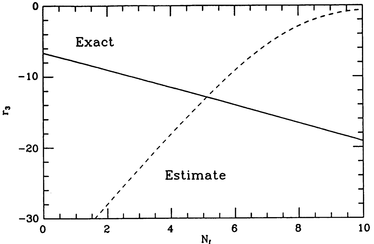
Figure 4.1 N_f dependences of exact result (4.45) and estimate (4.42) for r_3 .
