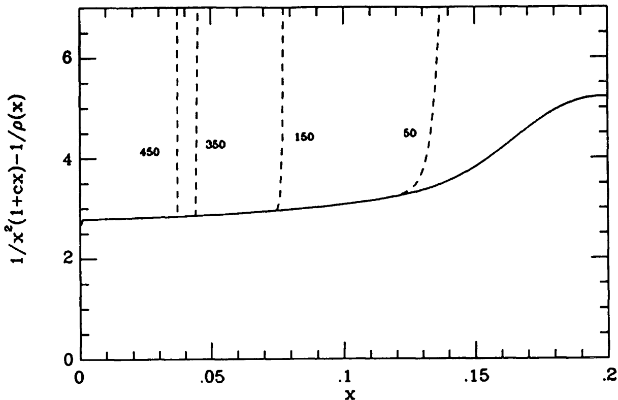
Figure 7.2 Numerical Results ( c > 0 )
