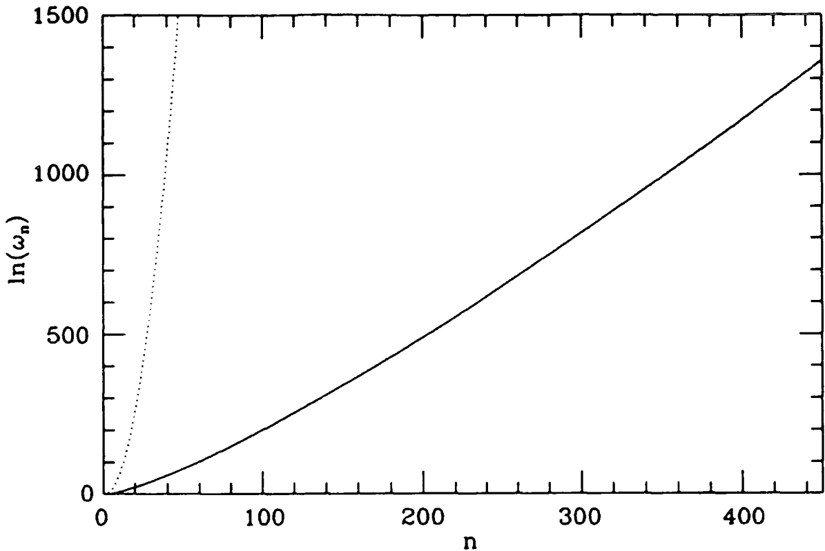
Figure 6.1 The series coefficients.
