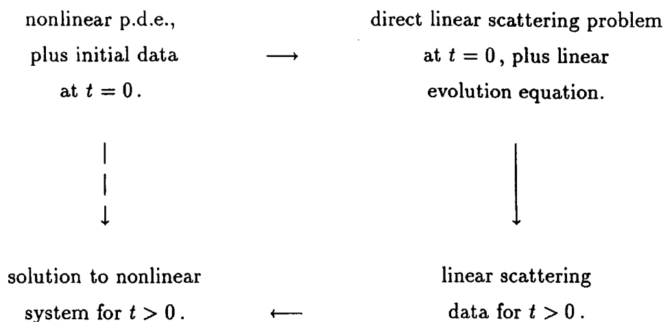
Fig 1.1. Flow diagram of the method of inverse scattering
