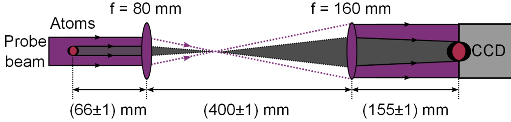
Figure 3.9: Schematic of the apparatus required to take an absorption image of the atoms. The probe beam illuminates the atom cloud, which absorbs some of the probe photons. Two achromatic doublet lenses magnify the absorption profile with a magnification of (1.858 \pm 0.002) (see figure 3.10). The probe beam is detected on a CCD camera. Diagram not to scale.
